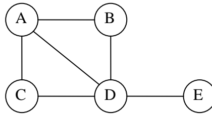
Figure 23 : Un graphe G(V, E)
