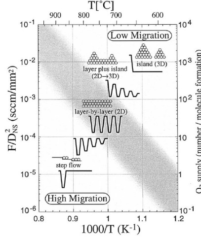
Figure 2.3: Phase diagram showing the growth mode of homoepitaxial SrTiO 3 as a function of the deposition parameters. For any growth mode the observed intensity modulation of the RHEED pattern is reported[30].
