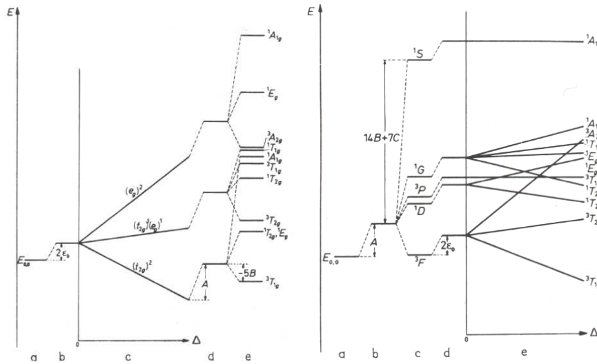
Figure 1.5: Left: splitting of the energy levels for a d^2 system in a strong octahedral field: a) d electron energy; b) ligand field destabilisation; c) ligand field splitting; d) electron-electron interactions. Right: splitting of the energy levels for a d^2 system in a weak octahedral field: a) d electron energy; b) c) electron-electron interactions; d) ligand field approximation; e) ligand field splitting. From ref. [3]
