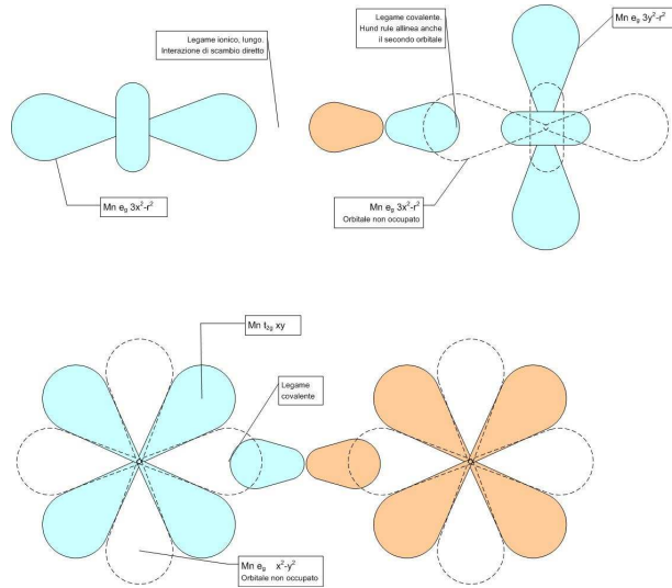
Figure 1.13: Goodenough rule for the oxygen mediated superexchange interaction between Mn ions. Top: semicovalent bond between Mn^{3+} ions in the orbital ordered phase. Bottom: covalent bond between Mn^{4+} ions (for example in CaMnO_3 that is a G-type AFM). Orange and blue fillings represent the spin orientation, the small orbital represents oxygen 2p .
