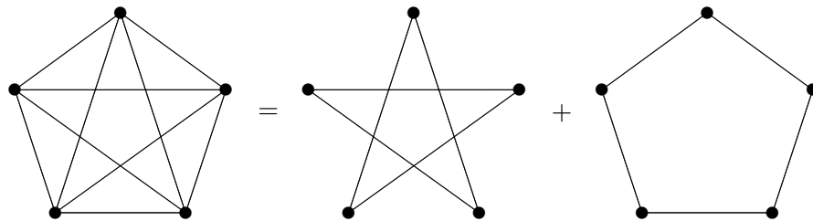
Figure 2.4: Non-induced C_5 -decomposition of K_5
