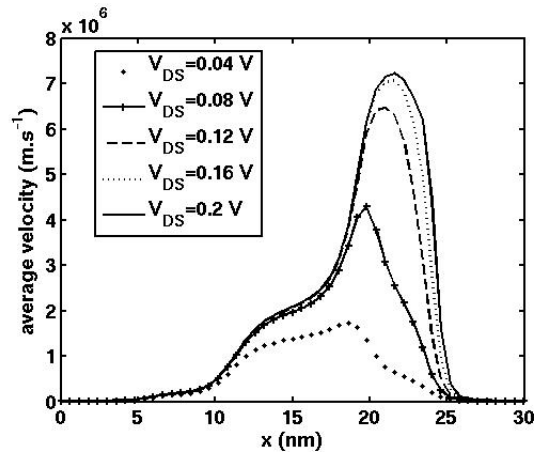
Figure 3.8: Average velocity ( m s^{-1} ) for V_G = -0.1 V.
