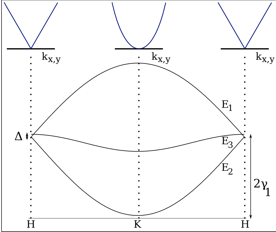
Figure 2.11 – The band structure along the \mathbf{H} – \mathbf{K} – \mathbf{H} -line. The dispersion of the E_1 and E_2 bands is 2\gamma_1 at the \mathbf{K} -point. \Delta shifts the E_3 band with respect to E_1 and E_2 at the \mathbf{H} -point. The in plane dispersions at the \mathbf{K} - and \mathbf{H} -points are added. Around the \mathbf{H} -point we find similar dispersion as for mono-layer graphene and thus the features of massless relativistic particles. Around the \mathbf{K} -point we find parabolic dispersion and similarity to bi-layer graphene. In bi-layer graphene the carriers behave like massive relativistic particles.
