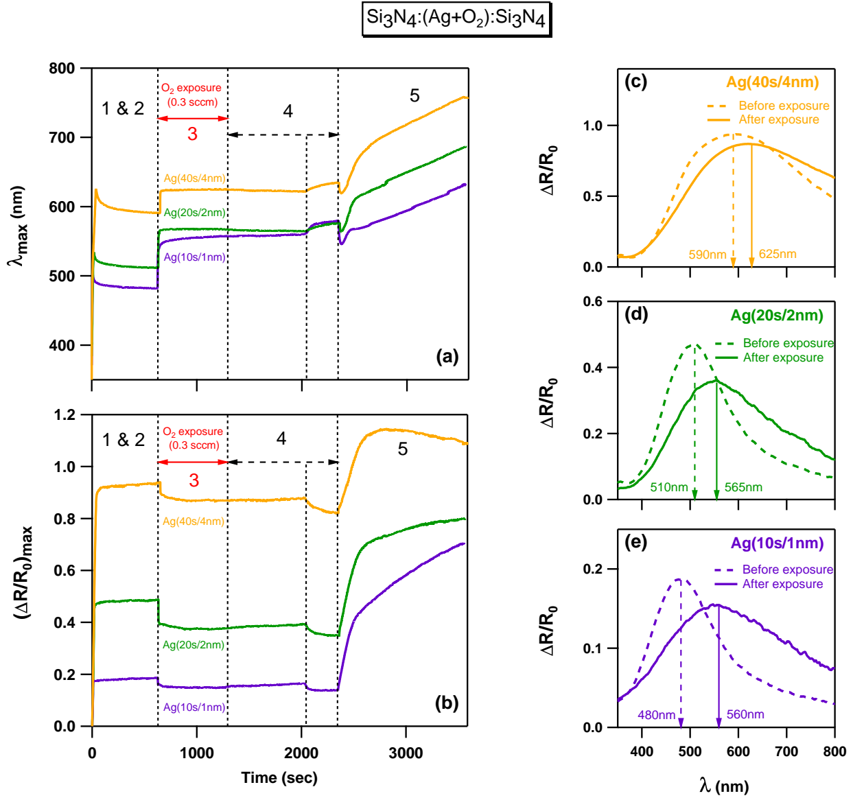
Figure IV.7 – Comparison for temporal variations of \lambda_{\max} (a) and (\Delta R/R_0)_{\max} (b) during the \text{Si}_3\text{N}_4:\text{Ag}:\text{Si}_3\text{N}_4 nanocomposite depositions with increasing Ag deposition time/amount (10s/1nm to 40s/4nm), Ag nanoclusters of which are exposed to \text{O}_2 . (c-e) represent the spectral variations in the SPR of the Ag nanoclusters before (around 600s - dashed curves) and after (around 1200s - solid curves) the exposure. The experimental details for each deposition step (from STEP 1 to STEP 5) are given in Table IV.2
