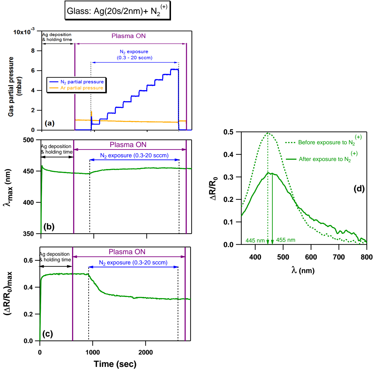
Figure IV.16 – (a): Temporal variation of N 2 partial pressure in the deposition chamber after the ignition of the Ar + plasma at the Si 3 N 4 target (Plasma ON), (b-c): temporal variations in λ max and (ΔR/R 0 ) max of glass Ag nanoclusters during their exposure to N 2 (+) , (d): the spectral SDRS signals before and after exposure of the Ag nanoclusters to the partially ionized N 2 .
