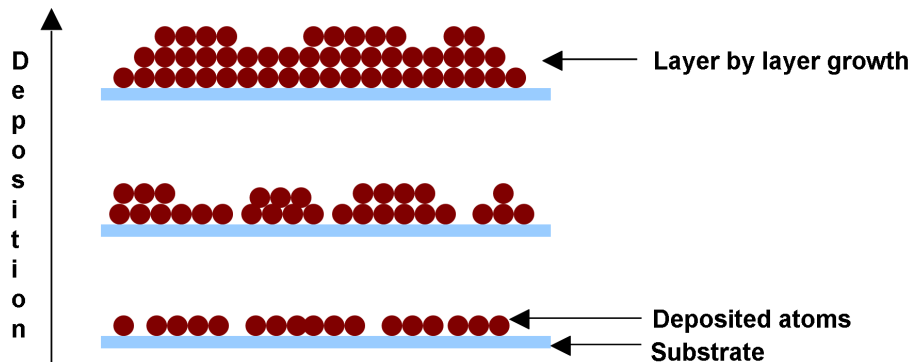
Figure I.5 – A 2D layer by layer or FM growth of the material on the substrate surface.
