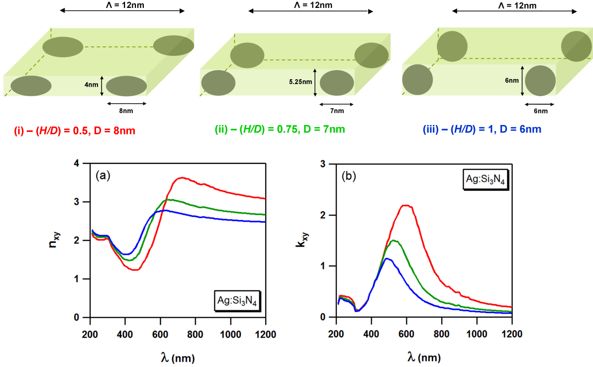
Figure A.7 – Effect of cluster shape H/D and cluster size D (i to iii) on the effective in-plane complex refractive index of Ag:Si 3 N 4 nanocomposites (a-b), considering the deposited Ag amount t_{\text{Ag}} and the inter-cluster distance \Lambda are constant.
