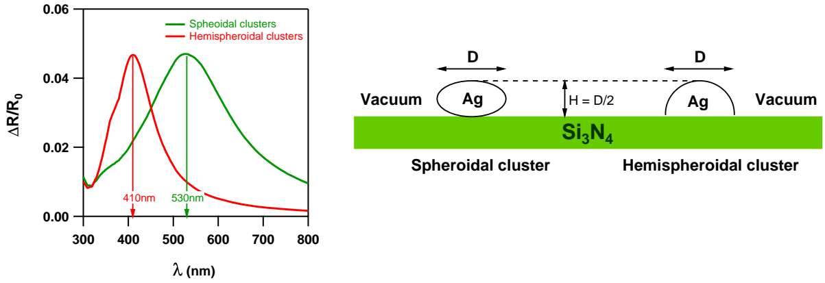
Figure II.14 – Simulations of \Delta R/R_0 (for s -polarized light and at an incidence angle = 70^\circ ) in case of Ag spheroidal nanoclusters surrounded by vacuum on a \text{Si}_3\text{N}_4 substrate with ellipsoidal or hemispherical shape.
