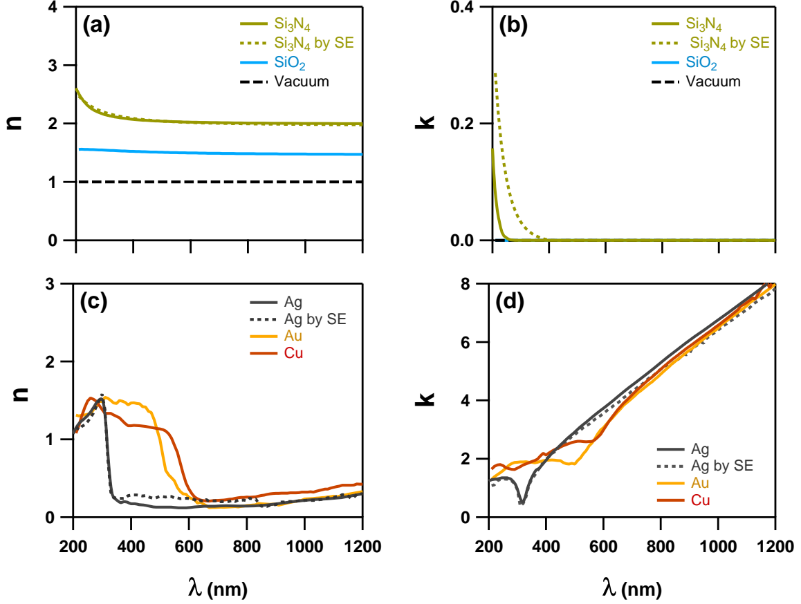
Figure II.1 – Tabulated values (continuous curves) for complex refractive indices n(\lambda)+ik(\lambda) of dielectric materials (a-b) and noble metals (c-d). SE measurements show confirmations of tabulated values in case of \text{Si}_3\text{N}_4 and Ag (dashed curves).
