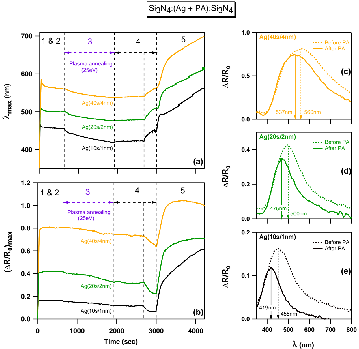
Figure V.9 – Temporal variations of \lambda_{\max} (a) and (\Delta R/R_0)_{\max} (b) for plasma annealed (PA at 25eV) Ag nanoclusters during the deposition of \text{Si}_3\text{N}_4:\text{Ag}:\text{Si}_3\text{N}_4 nanocomposites with increasing Ag amounts (10s/1nm, 20s/2nm, and 40s/4nm). (c-e) represents the spectral variations in the SPR of the Ag nanoclusters before (around 650s - dotted curves) and after (around 1920s - thick curves) the plasma annealing for respective samples during STEP 3 (attention for the scale).
