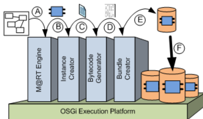
Figure 6.12: Instance creation tool chain
