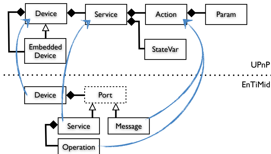
Figure 8.7: Mapping UPnP-EnTiMid
