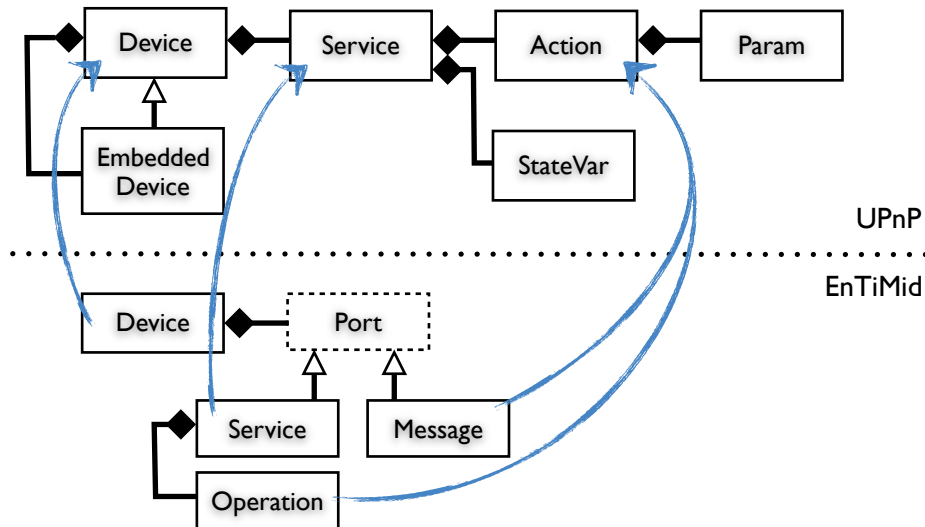
Figure 8.7: Mapping UPnP-EnTiMid
