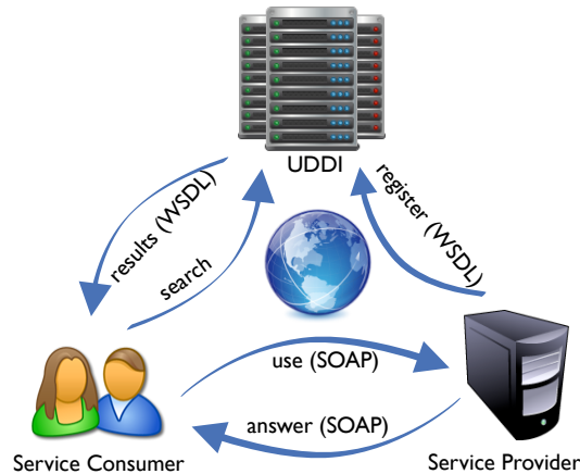
Figure 3.2: WebService Architecture
