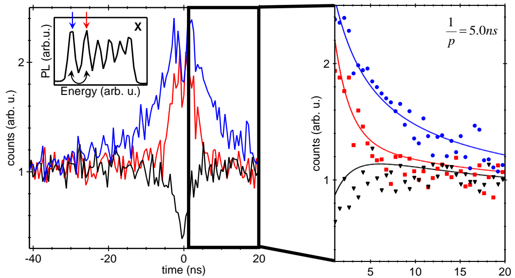
Figure 5.6: Comparison of the results of the auto- and cross-correlation measurements (points on the right panel) with the model described in text using the time constant of the Mn^{2+} spin flips as a fitting parameter.
