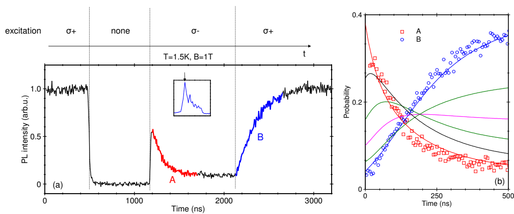
Figure 5.13: (a) The temporal profile of the intensity of one of the six excitonic lines (marked in the inset) under the excitation pattern shown in the upper part of the figure and described in the text. (b) Calculated temporal profiles of occupation of six \text{Mn}^{2+} spin states after the rapid change of excitation from one circular polarization to the opposite one (solid lines) compared with the temporal profiles of occupation of the extreme state measured in the experiment (symbols).
