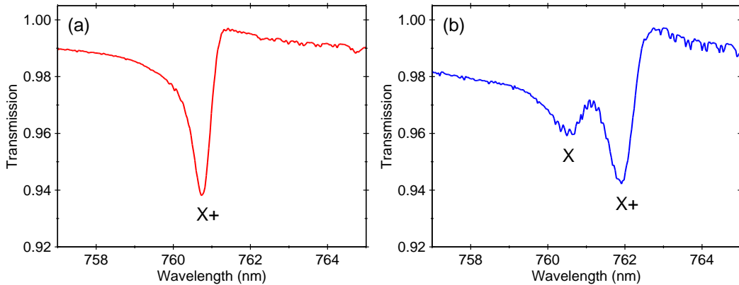
Figure 2.3: Transmission spectra of a p -type sample containing a CdTe quantum well doped with 0.8% of Mn: (a) with illumination with long-wavelength-pass filter (high density of hole gas) (b) with illumination with white lamp without any filter (low holes density)
