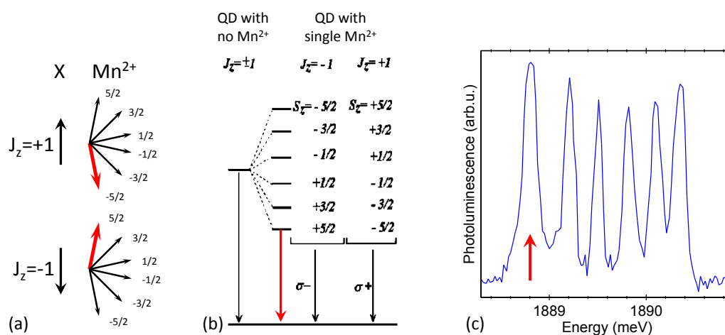
Figure 1.10: (a) Schematic diagram of possible relative orientations of the exciton and \text{Mn}^{2+} spin. Numbers indicate spin projection onto the quantization axis parallel to the growth axis of the sample. (b) Diagram of the neutral exciton energy levels and optical transitions in the non-magnetic quantum dot (left) and in the single Mn-doped dot (right). (from Ref. [49]) (c) Photoluminescence spectrum of the neutral exciton confined in the quantum dot with single \text{Mn}^{2+} ion taken without polarization resolution. Red arrows indicate the spin states and photoluminescence line related to each other.
