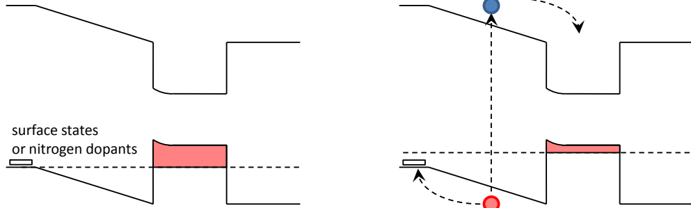
Figure 2.2: Schematic diagram of the mechanism allowing the control over the hole gas density in the quantum well in the p -type samples. The change in carrier density is obtained by illuminating the sample with light of energy above barrier band gap. Blue colour refers to electrons, the red one to the holes.
