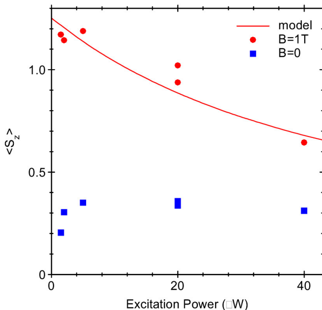
Figure 5.12: The mean spin of the \text{Mn}^{2+} ion as a function of excitation power for B=0 and B=1 T compared with model described in text (solid line).
