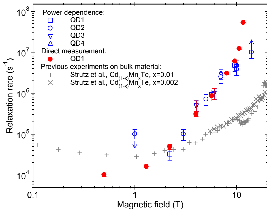
Figure 7.9: Spin-lattice relaxation rate of a single Mn^{2+} ion in the quantum dot as a function of magnetic field, measured for several dots (colour points) using two different methods described in text in comparison with the relaxation rate measured in diluted Cd_{1-x}Mn_xTe bulk material (black points)
