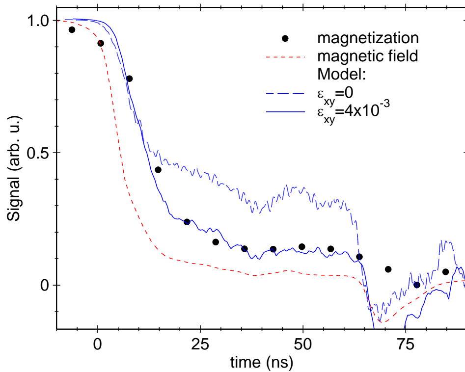
Figure 7.10: Magnetization dynamics of a Cd 1-x Mn x Te quantum well with 0.8% of Mn at B = 0 after the pulse of magnetic field (symbols), coil current (dotted line), and the result of calculations (solid and dashed lines) described in the text.
