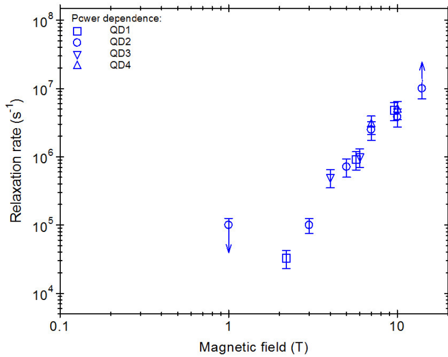
Figure 7.3: Spin-lattice relaxation rate of a single Mn 2+ ion in the quantum dot as a function of magnetic field, measured for several dots.
