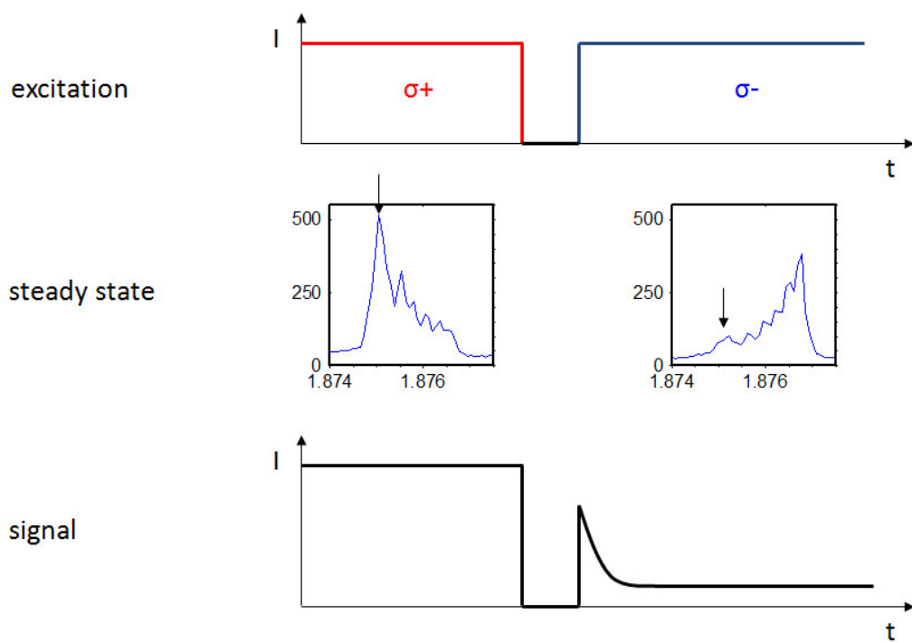
Figure 7.4: The idea of the direct measurement of the spin relaxation time of a single Mn^{2+} ion in the quantum dot for low magnetic field
