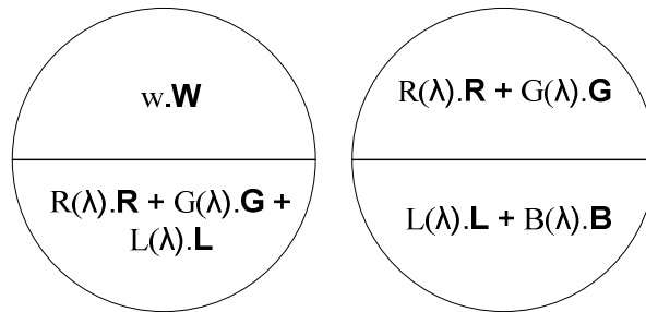
Fig. 2-11. Color-matching by the Maxwell method (left) and the maximum saturation method (right) ([9], page 384)
