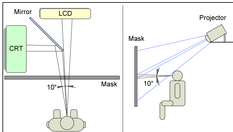
Fig. 5-33. Experimental setup
