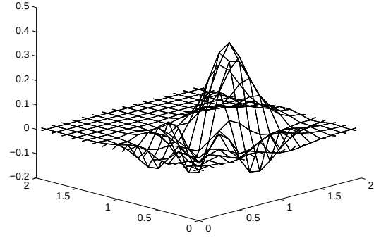
FIGURE 2 – The oscillating solution at time t = 1 using the centered scheme with h_D = 0.1768
