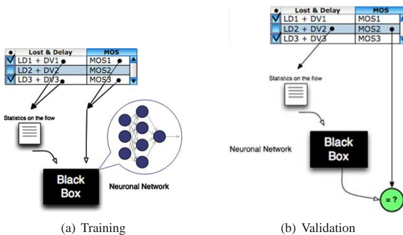
Figure 3.5: Learning of the quality behavior with RNN.
