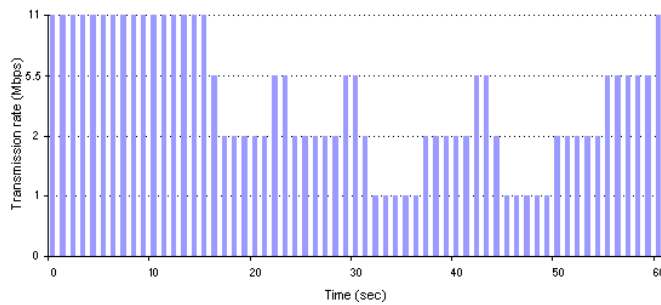
Figure 5.10: Rate adaptation of the proposed scheme during the test scenario.
