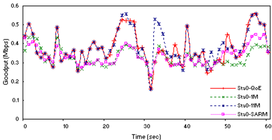
Figure 5.8: Goodput of a fixed station.
