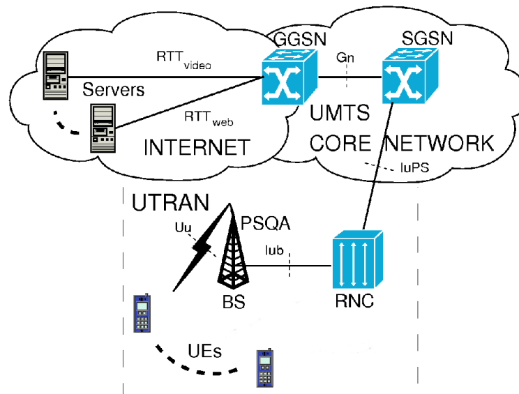
Figure 6.1: Simulation topology.
