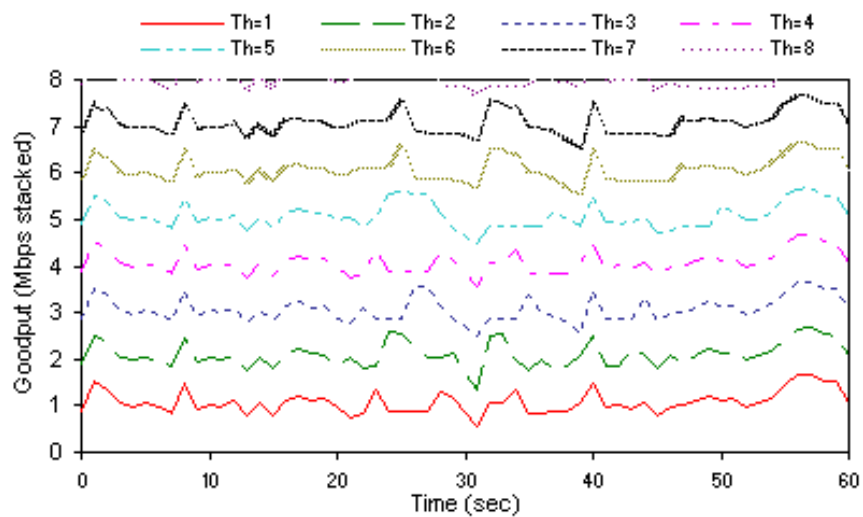
Figure 5.6: Goodput for different values of threshold.
