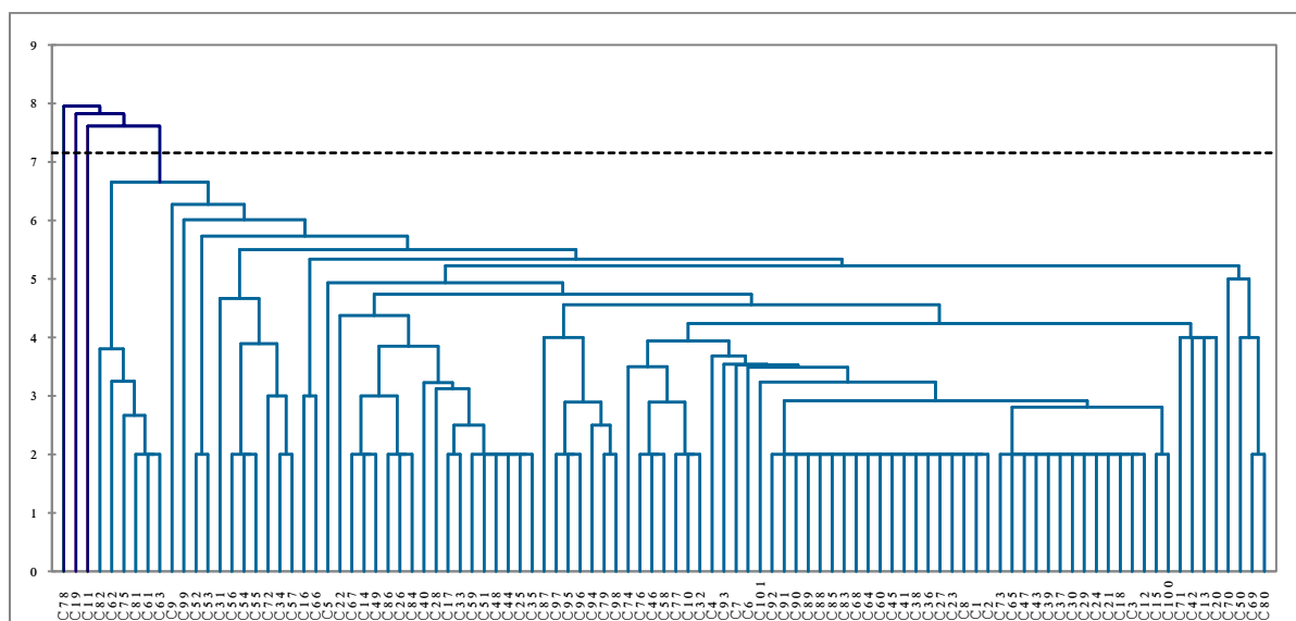
Figure 4.14 – Dendrogramme, G = 10 ; V = 7,155
