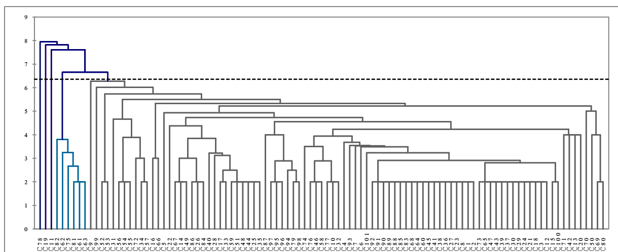
Figure 4.13 – Dendrogramme, G = 20 ; V = 6,36
