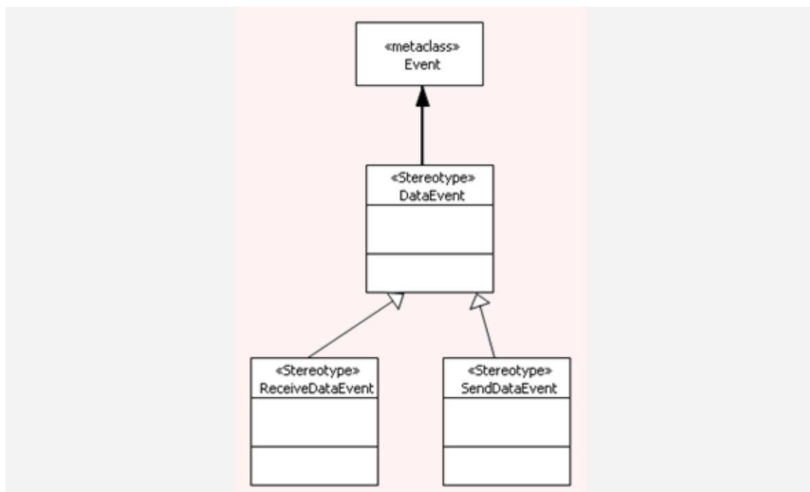
Figure 17 Definition of the DataEvent concept
