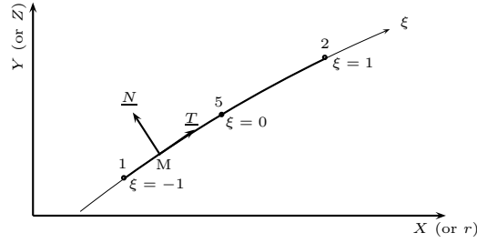
Figure A.4: Local coordinates of the reference curve
