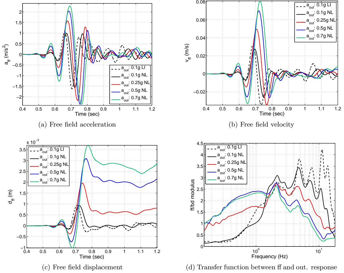
Figure 5.13: First second of the response in terms of free field acceleration, velocity and displacement for the soil profile #3 and the transfer function between the free field response and the outcropping for different input motions
