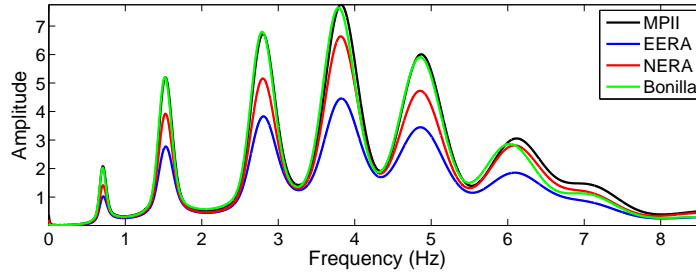
Figure 3.24: Transfer function of the acceleration between the surface of the three-layer soil column (#2) for applied Ricker wavelet of order zero at the base of the soil layer (boundary condition in displacement) equivalent to a 0.015g outcrop PGA
