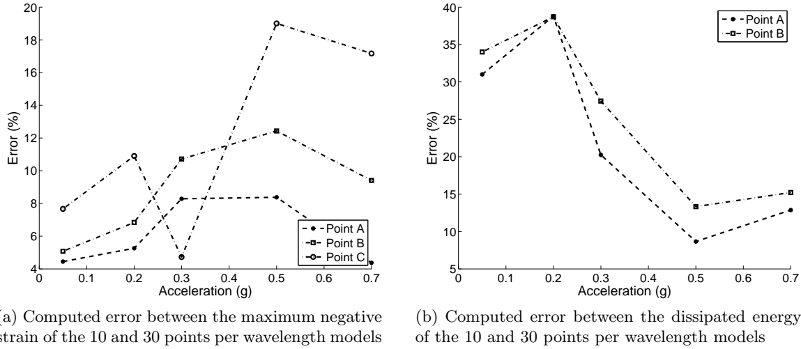
Figure 4.29: Computed error of the maximum negative strain (left) and the dissipated energy (right) during the propagation of the 10 and 30 points per wavelength models versus the five different input motions (acceleration) for the three selected control points (A, B and C) and the 10-spring constitutive model
