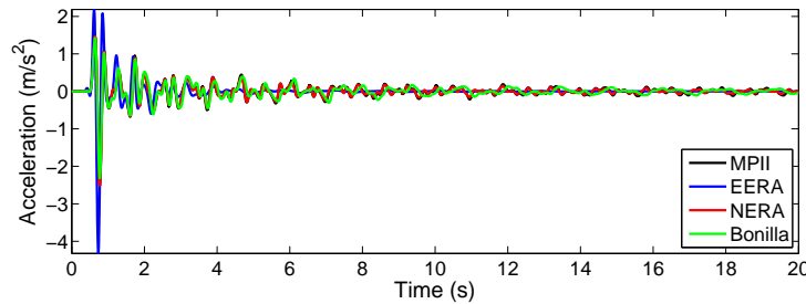
Figure 3.20: Acceleration obtained at the surface of the three-layer soil column for applied Ricker wavelet of order zero at the base of the soil layer (boundary condition in displacement) equivalent to 1.0g outcrop PGA
