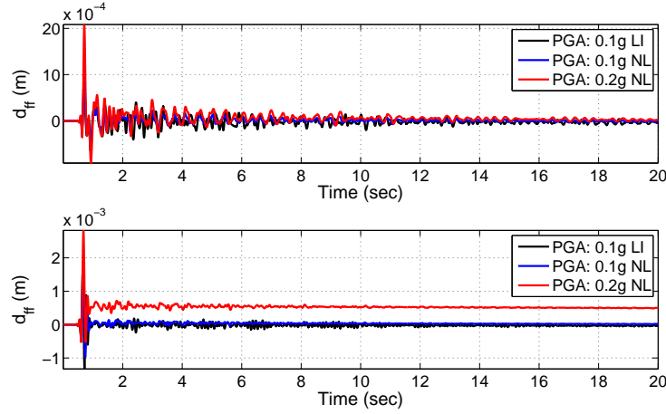
Figure 6.16: Comparison between the basin responses (displacement) due to different soil behaviors and input motions at the points N_1 (top) and N_2 (bottom)
