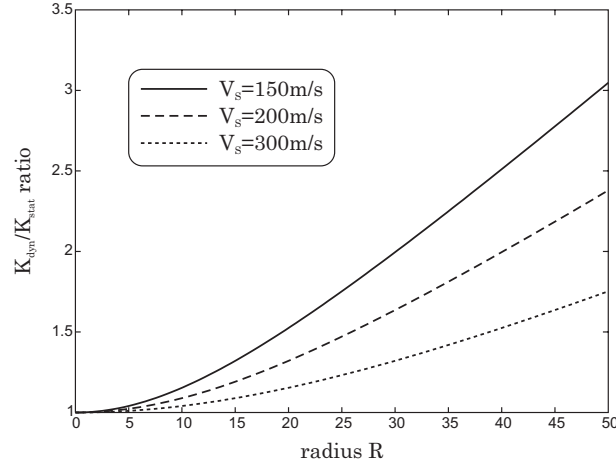
Figure 1.7: K_{dyn}/K_{stat} ratio estimated through cone models as a function of the foundation radius R for various shear wave velocities: V_S = 150 m/s, V_S = 200 m/s and V_S = 300 m/s ( \nu = 0.25 , \mu = 200 MPa and f = \frac{\omega}{2\pi} = 2 Hz).
