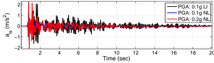
Figure 6.17: Acceleration at the top of the structure for different soil behaviors and input motions
