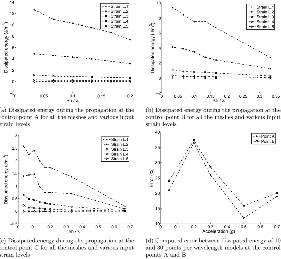
Figure 4.26: Dissipated energy for each stress-strain curves of 8 meshes at the three different control points (A, B and C) for the 50-spring model for 5 different strain input levels and the calculated error between dissipated energy of 10 and 30 points per wavelength models at the control points A and B versus related input maximum acceleration (bottom-right)
