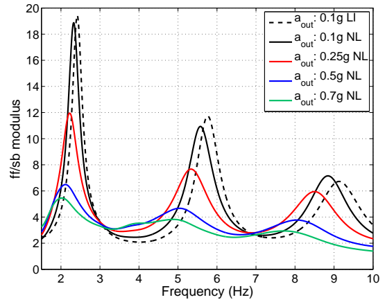
(b) Transfer function of ff/bs for soil profile #2
