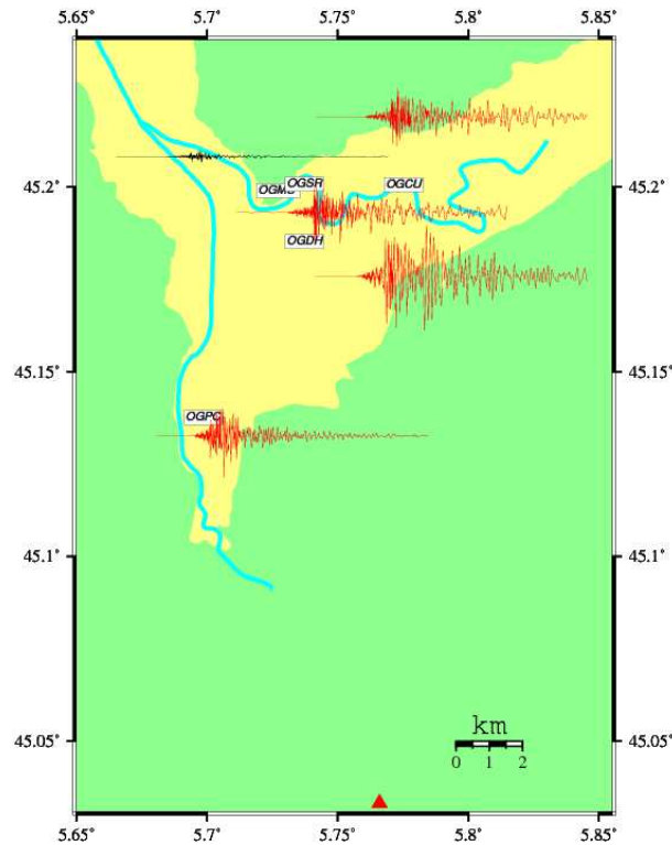
Figure 1.2: Velocities ( N - S component) recorded at various locations in the city of Grenoble during the 1999 Laffrey earthquake (data: French accelerometric network, www-rap.obs.ujf-grenoble.fr , reference: (Lebrun et al., 2001)).
