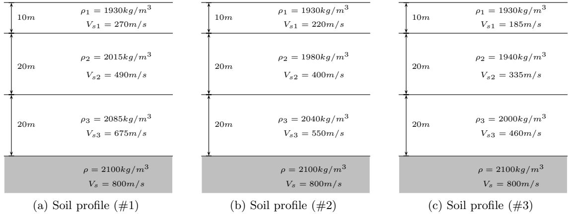
Figure 5.2: Geometric and material properties of the three selected soil profiles
