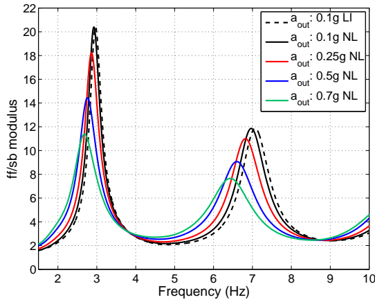
(a) Transfer function of ff/bs for soil profile #1
