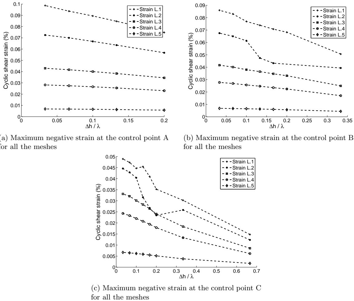
Figure 4.24: Maximum negative strain at the three different control points of the model (A, B and C) for all the meshes for the 50-spring constitutive model and the various input strain levels
