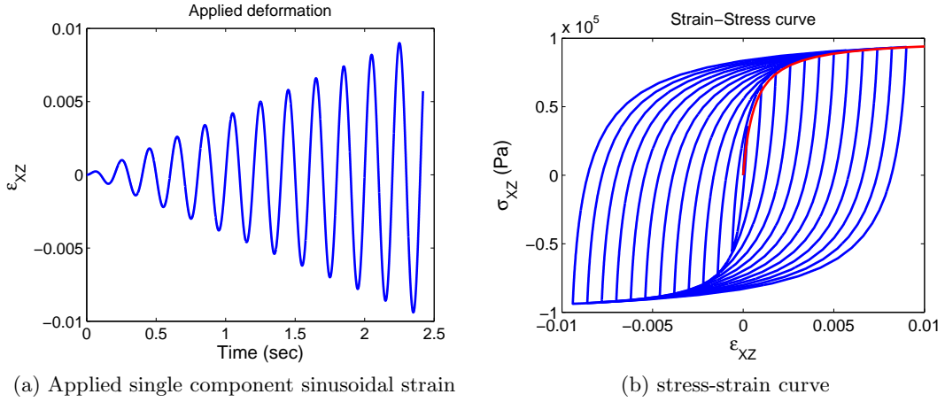
Figure 4.5: Applied single component sinusoidal strain (left) and the stress-strain curve obtained using the implemented MPII model (right)
