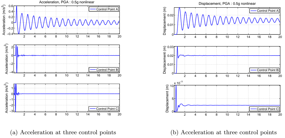
Figure B.7: Horizontal acceleration and displacement for three control points A, B and C of structure 7 (PGA: 0.5g)
