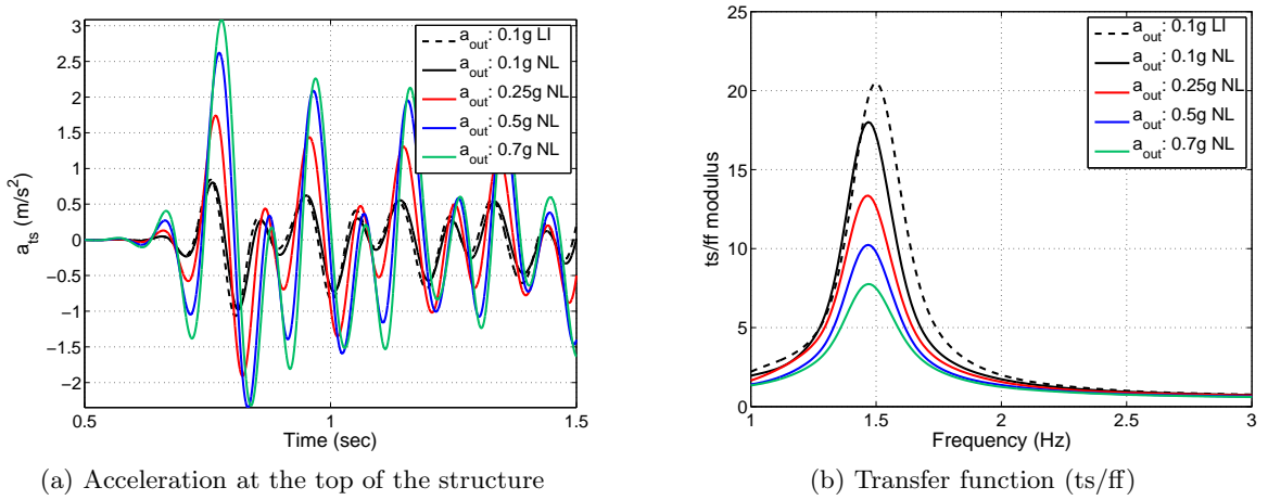
Figure 5.27: Acceleration at the top of the structure (left) and the transfer function (right) between the acceleration at the top of the structure and the free field for the case study 8 (see Table 5.5)
