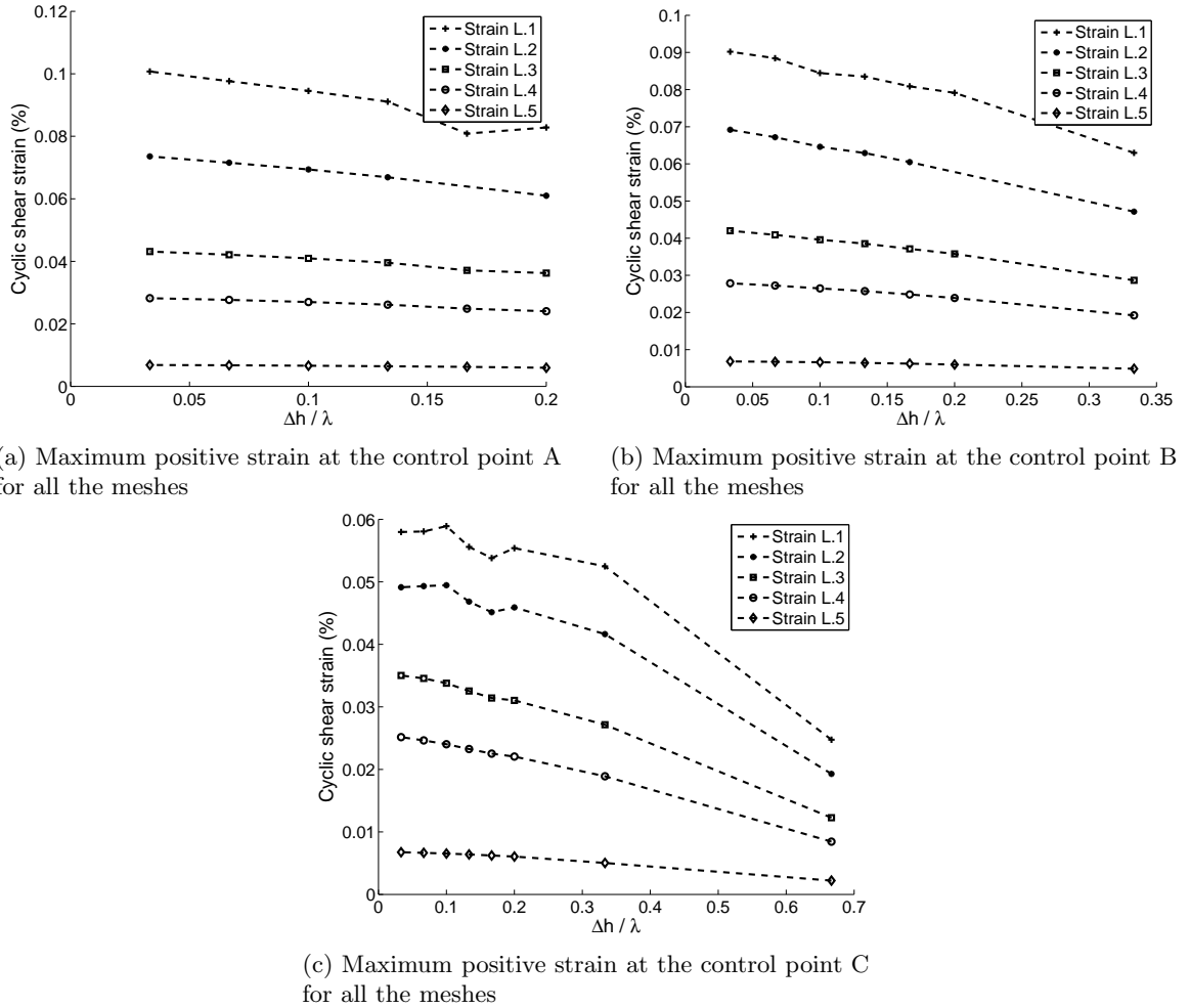
Figure 4.23: Maximum positive strain at the three different control points of the model (A, B and C) for all the meshes for the 50-spring constitutive model and the various input strain levels
