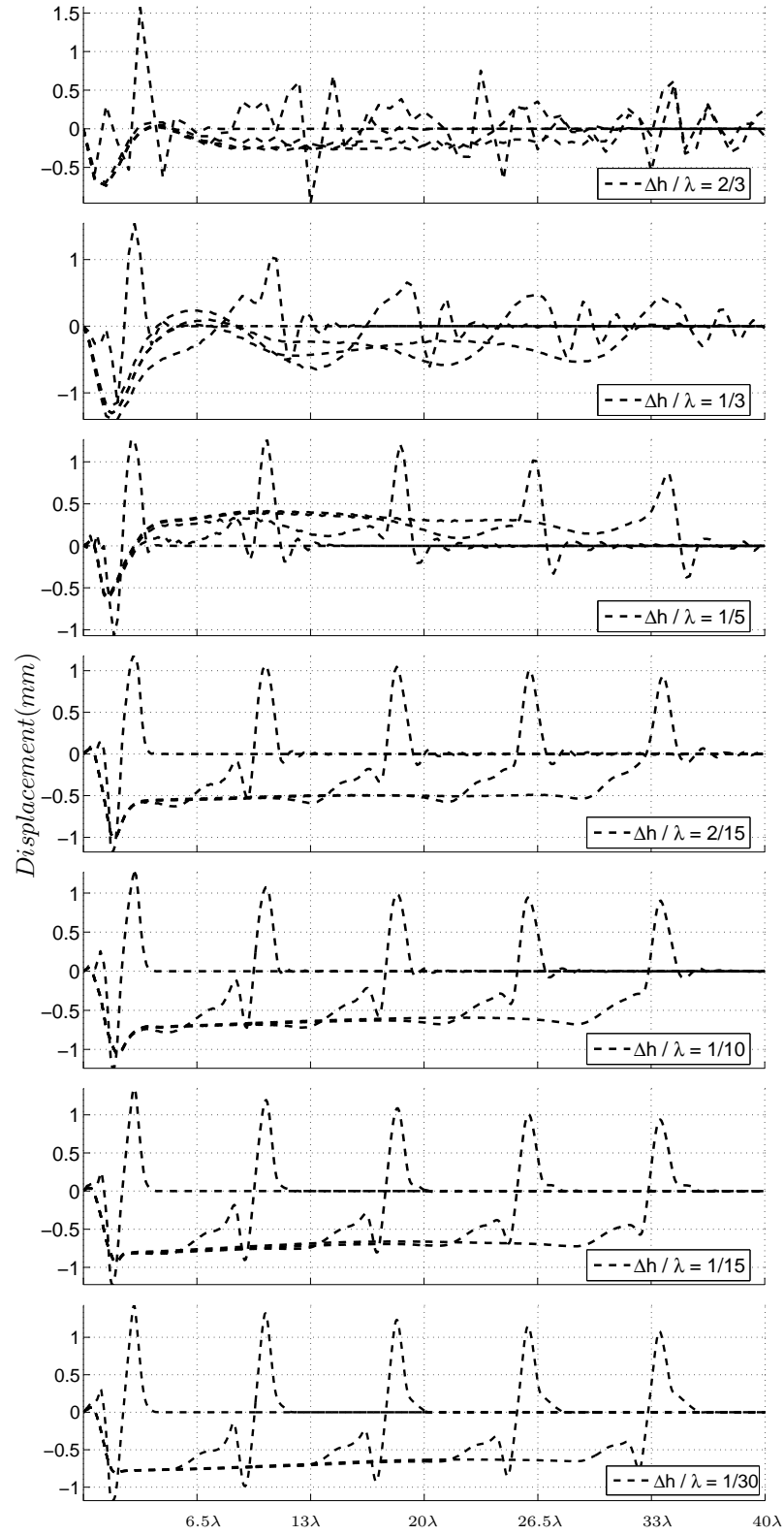
Figure 4.9: Wave forms (displacements) for different models at various times in the 40\lambda nonlinear medium considering a 5-spring MPII model
