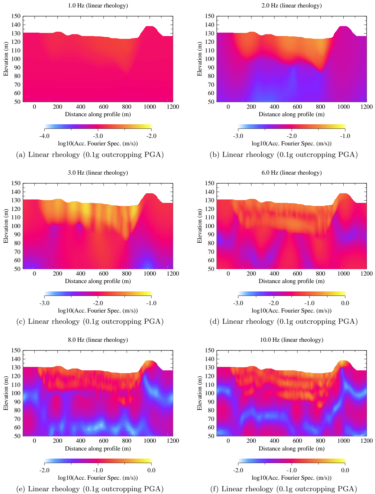
Figure 6.6: Acceleration Fourier spectrum for linear soil rheology at 0.1g outcropping PGA's
