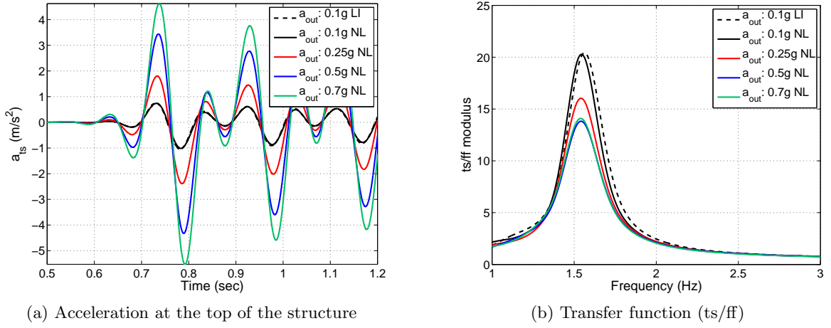
Figure 5.26: Acceleration at the top of the structure (left) and the transfer function (right) between the acceleration at the top of the structure (ts) and the free field (ff) for the case study 7 (see Table 5.5)
