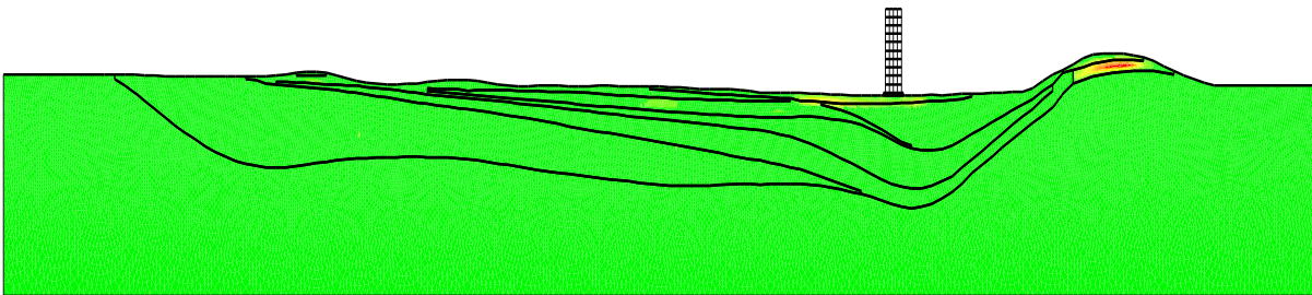
Figure 6.21: Cumulative dissipated energy into the basin due to the shear stress components for 0.1g outcropping PGA (different horizontal and vertical scales)
