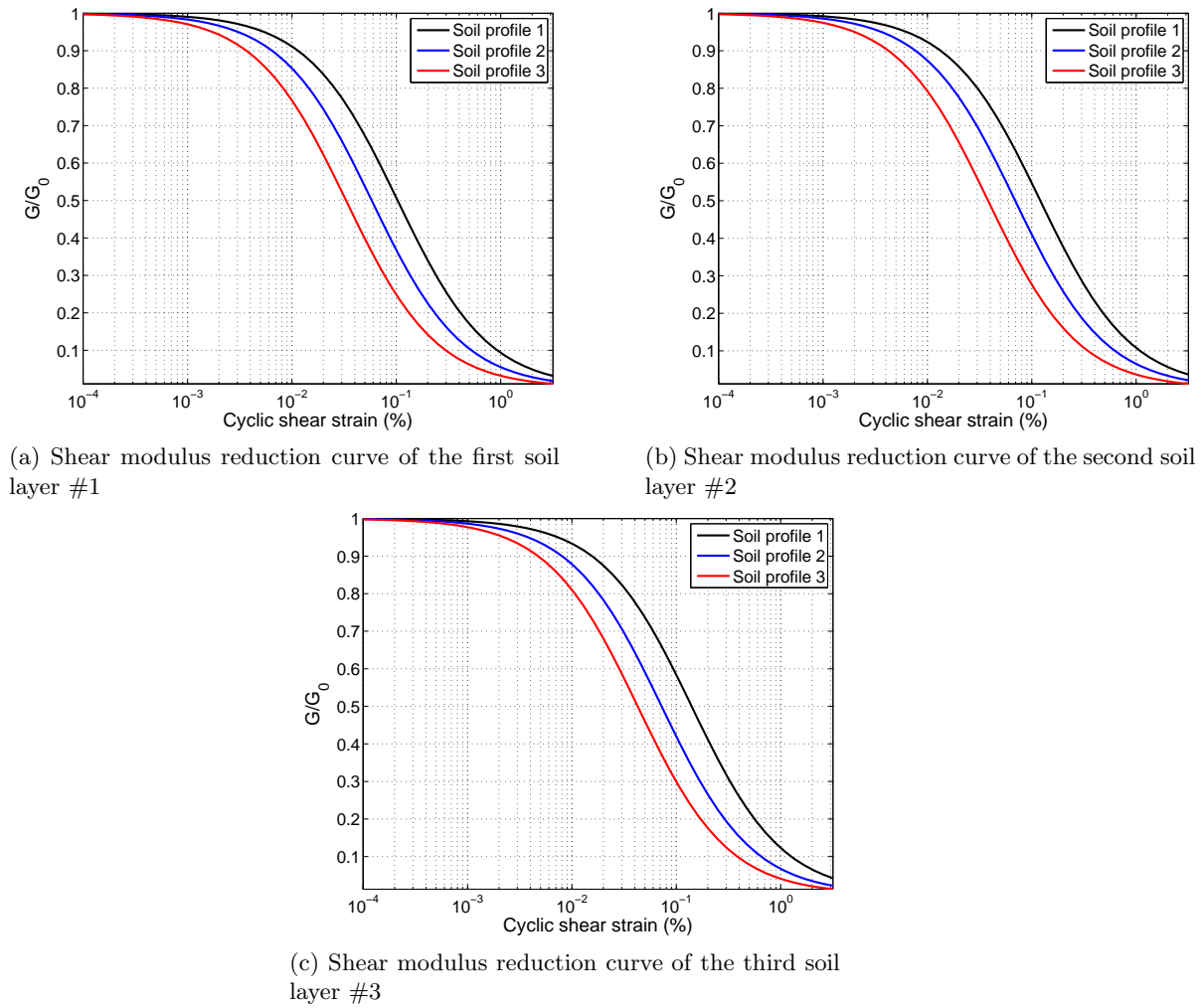
Figure 5.5: Shear modulus reduction curve for the three selected soil profiles
