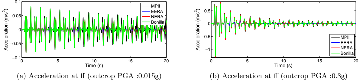
Figure 3.14: Acceleration at the surface of the soil column excited by a Ricker wavelet of order zero at the base of the soil layer for two different input levels (equivalent to 0.015 and 0.3g outcrop PGA)
