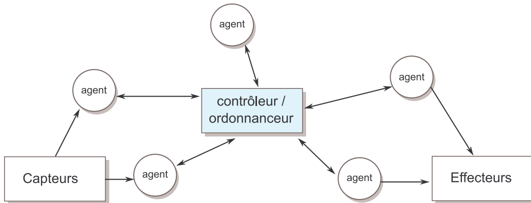
FIGURE 1.7 – Architecture multi-agent
