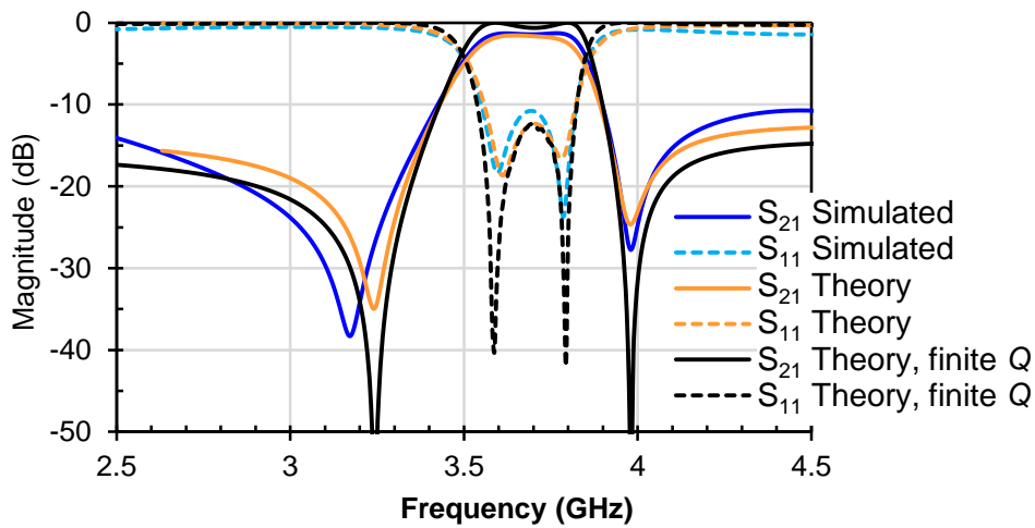
Figure 28 – Theoretical curves from (34), considering a resonator with infinite Q and finite Q = 80 .
