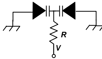
Figure 23 – Back-to-back configuration of the varactor diodes to allow biasing and improve linearity.
