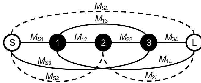
Figure 6 – Coupling scheme of a 3 rd -order filter considering all possible couplings. Source and load are represented by white circles and resonators represented by black circles.
