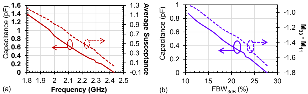
Figure 62 – Simulated and theoretical curves of the filter loaded with equal capacitances at the four slots (a) center frequency x capacitance (full-line), center frequency x average susceptance (dashed-line); (b) bandwidth x capacitance (full-line), bandwidth x (M_{33} - M_{11}) (dashed-line).
