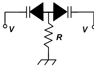
Figure 55 - Back-to-back configuration of the varactor diodes to halve the capacitance and improve linearity.
