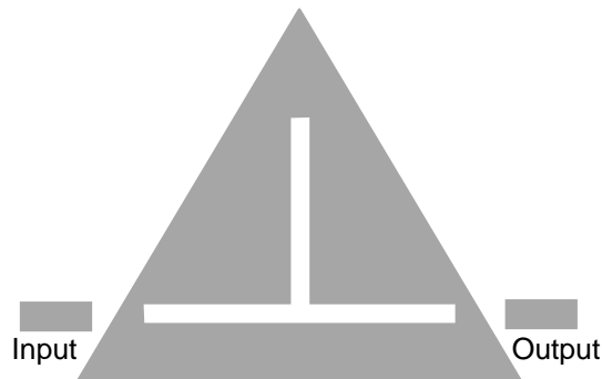
Figure 13 – Layout of the triangular patch resonator weakly coupled to the input and output, with a vertical and a horizontal slot.
