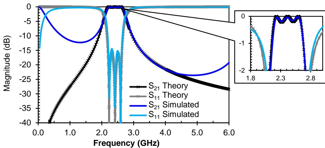
Figure 50 – Lossless simulated and theoretical (from matrix M_o in (43)) responses of the unloaded triple-mode circular patch filter. An inset of the passband is shown on the upper right corner.
