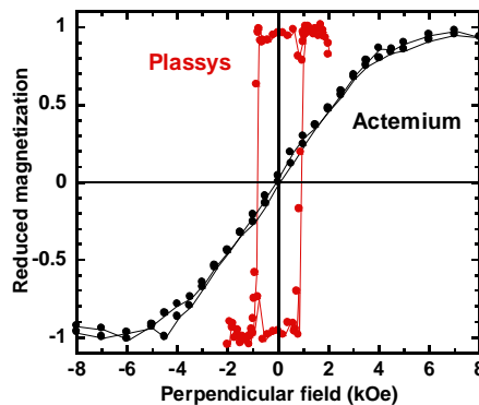
Figure I-18: Reduced magnetization as a function of perpendicular magnetic field, after annealing at 300°C, in two Ta 3 /Pt 30 /Co 0.5 /CoFeB 1 /MgO 2 RF structures deposited in our Actemium (black) and Plassys (red) sputtering units.
