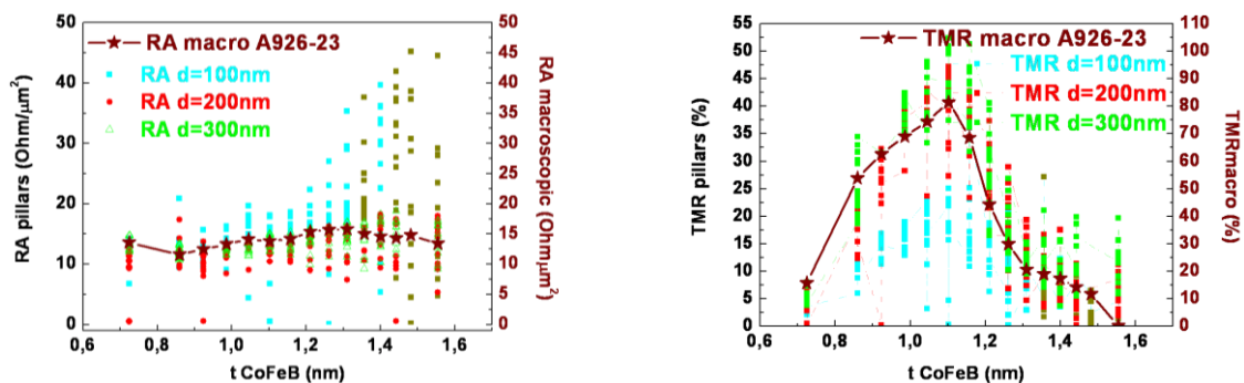
Figure IV-9: RA product (left) and TMR ratio (right) as a function of CoFeB thickness for 100, 200, 300nm pillars, and comparison with macroscopic (Capres) measurements.
