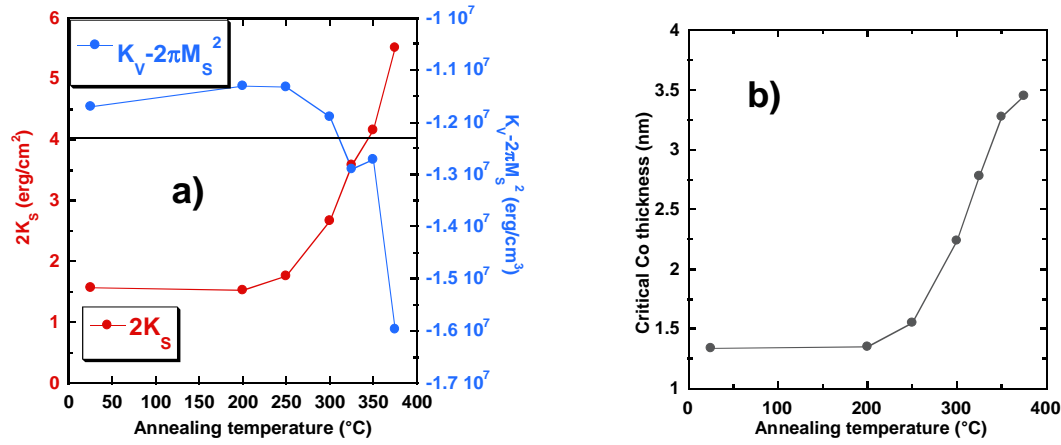
Figure I-14: (a) Interface and volume anisotropies as a function of annealing temperature in Ta3/Pt20/Co/Mg1.4NatOx/Cu2/Pt2 structures. The horizontal line corresponds to -2\pi M_S^2 , where M_S is the Co saturation magnetization ( 1400 \text{ emu/cm}^3 ); (b) Critical Co thickness as a function of annealing temperature.
