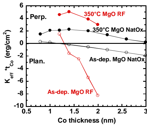
Figure I-15: Plots of K_{\text{eff}} \cdot t_{\text{Co}} as a function of t_{\text{Co}} before and after annealing at 350^\circ\text{C} in Ta3/Pt20/Cox/Mg1.4NatOx/Cu2Pt2 (black) and Ta3/Pt20/Cox/MgO1.6RF (red) structures.
