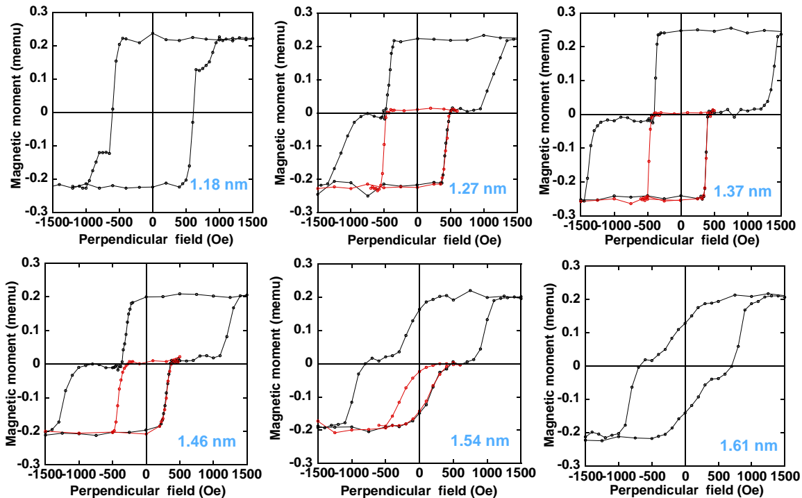
Figure II-45: Hysteresis loops of Ta3/Pt20/Co1.2/MgO/Co1.2/Pt3.0 perpendicular junctions as a function of Mg thickness after annealing at 270°C.
