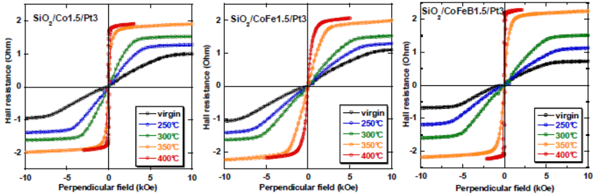
Figure I-24: Variation of the Hall resistance as a function of perpendicular magnetic field in \text{SiO}_2/\text{MM}1.5/\text{Pt}3 structures for different annealing temperatures. MM stands for Co (left), \text{Co}_{90}\text{Fe}_{10} (middle) and \text{Co}_{60}\text{Fe}_{20}\text{B}_{20} (right).
