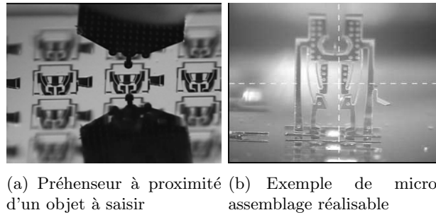
FIGURE 2.17 – Micropinche passive monodigitale (ARRI institute, Texas, USA, [40])
