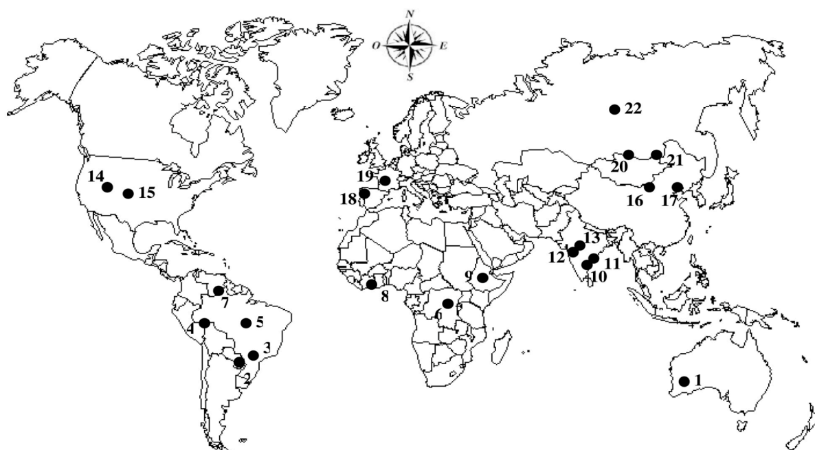
Figure 1. Localization of 22 grid cells on global map.
