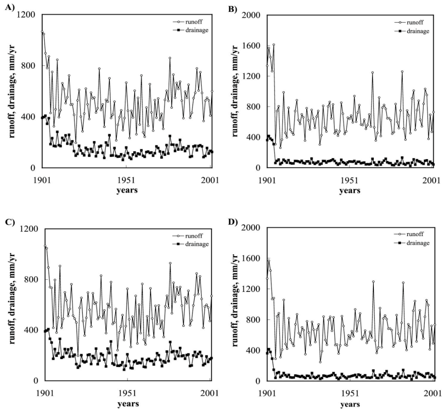
Figure 2. Drainage and surficial runoff in mm/yr calculated by LPJ model for a grid cell located in France (grid cell 19) for atmospheric CO 2 concentrations of (a) 355 ppmv and (b) 1120 ppmv and for a grid cell located in South America (grid cell 3) for atmospheric CO 2 concentrations of (c) 355 ppmv and (d) 1120 ppmv over the 1901–2002 period.
