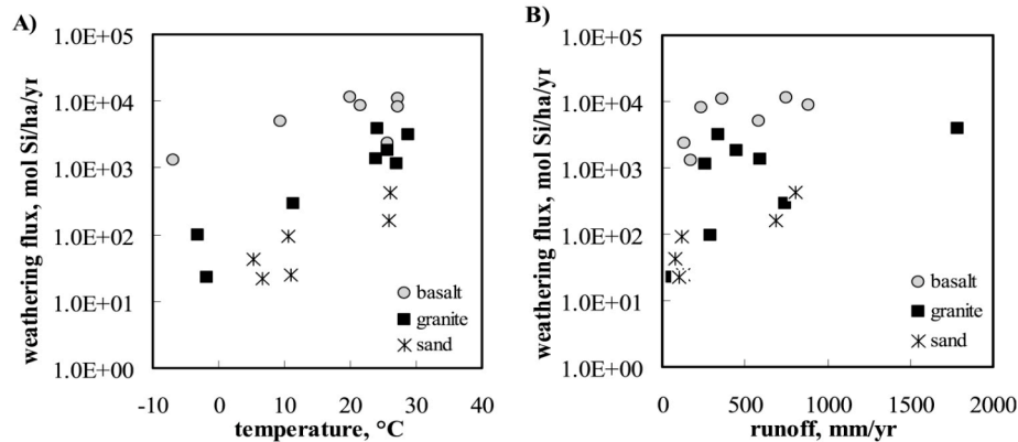
Figure 8. Calculated weathering flux in mol Si ha -1 yr -1 (a) versus temperature in degrees Celsius and (b) versus runoff in mm yr -1 for basaltic (gray circles), granitic (solid squares), and sandy (stars) lithologies. The temperature is the mean value over the 1982–2002 period, and the runoff is calculated by the LPJ model.
