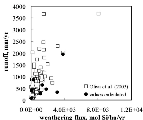
Figure 6. Runoff in mm yr -1 versus weathering flux in mol Si ha -1 yr -1 for granitic grid cells. The runoff is calculated by LPJ, and weathering flux is calculated by WITCH (solid circles). Field data from Oliva et al. [2003] (open squares).
