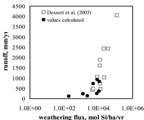
Figure 7. Runoff in mm yr -1 versus weathering flux in mol Si ha -1 yr -1 on basaltic rock. The runoff is calculated by LPJ, and weathering flux is calculated by WITCH (solid circles). Field data from Dessert et al. [2003] (open squares).
