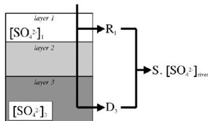
Fig. 3. B-WITCH model representation of the water fluxes and the sulfate ions concentrations for each grid element. [\text{SO}_4^{2-}]_1 and [\text{SO}_4^{2-}]_3 represent the surficial and deep \text{SO}_4^{2-} concentrations (mol/L) respectively, [\text{SO}_4^{2-}]_{\text{river}} is the \text{SO}_4^{2-} concentration into the river (mol/L), R_1 is the surficial runoff (mm/yr), D_3 is the deep drainage (mm/yr), and S is the river water flow (sum of deep drainage and surficial runoff).
