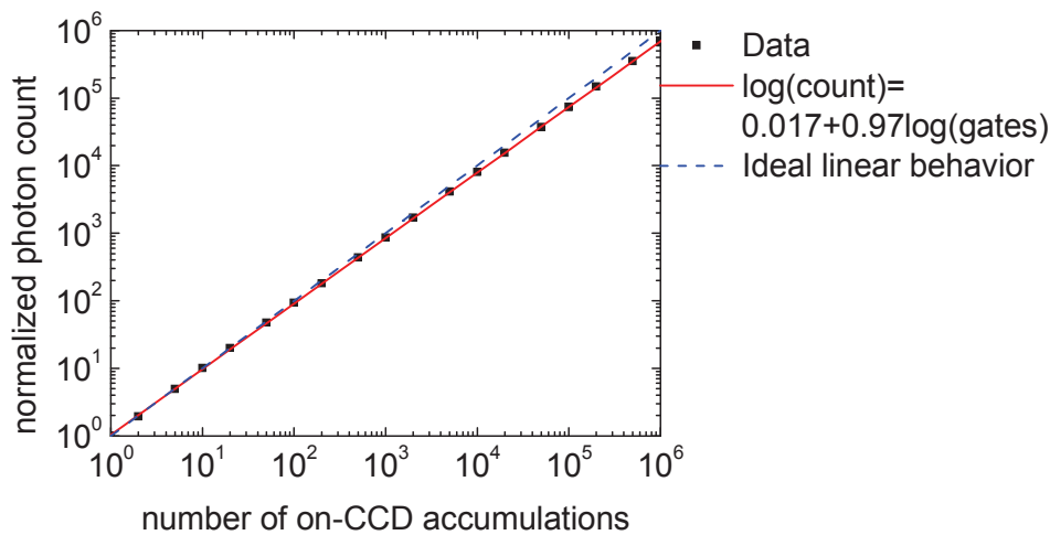
Figure 3.14. Measured photon count as a function of the number of on CCD accumulations (symbols) compared to ideal linear behavior (dotted line) taken from Pai, 2008
