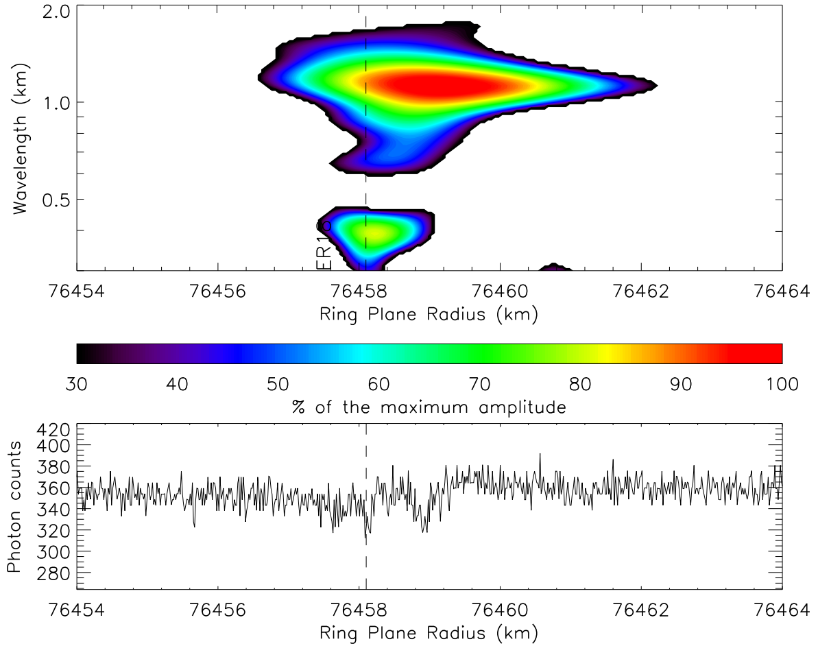
FIGURE 2.8 – Co-added WWZ wavelet power profile of embedded ringlet ER18, computed from individual occultation profiles. Lower panel shows the \beta Centauri, rev. 104 occultation profile. Two peaks, separated by 0.8 km, are visible on the occultation profile.
