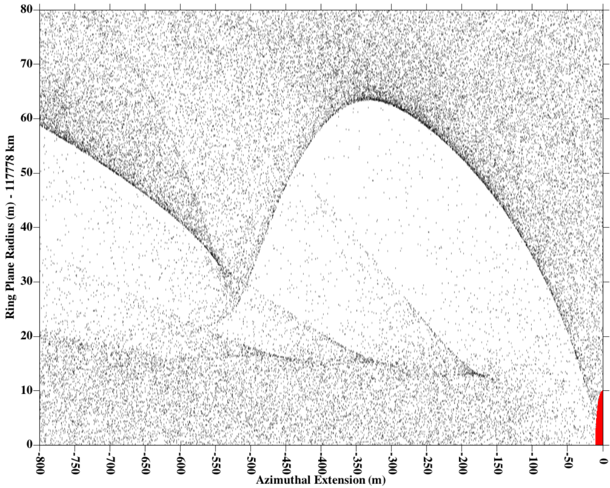
FIGURE 5.16 – Primary lobe of the propellers created by the interaction of 20-cm radius particles with a 10-m radius boulder. This zoom in is showing the primary trailing outer lobe of the depletion zone. Particles around this zone had a close encounter with the boulder less than one orbit ago.
