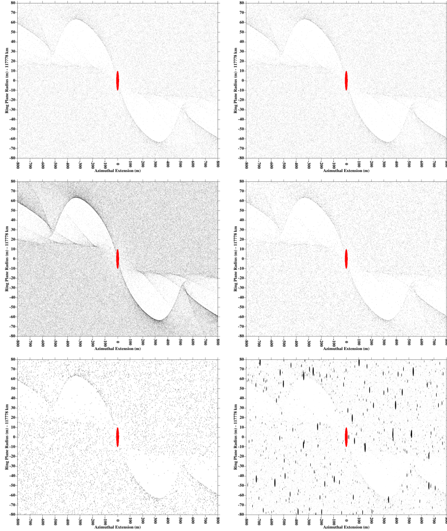
FIGURE 5.23 – Propeller signature for a 10-m radius boulder (represented in red). For left to right and top to bottom, particles radii are 5 cm, 10 cm, 20 cm, 50 cm, 1 m and following a power-law distribution with an index q = 2.75 reflecting the estimated Cassini Division particle distribution, between 10 cm and 1 m in the lower right panel. Optical depth is 0.1. Saturn’s direction is towards the bottom. Simulations involving 5-cm and 10-cm particles are too heavy and required being adapted as detailed in Section 5.3.2.3.2: we considered 40-cm particles instead with densities of 1.66 \text{ kg m}^{-3} in the first case and 13.3 \text{ kg m}^{-3} in the second one.
