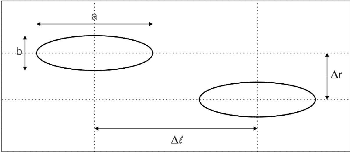
FIGURE 5.13 – The propeller model described by Equation 5.8. The coordinate system is a radius-azimuth grid, in which the direction toward Saturn is down (-r) and the orbital direction is to the right (+). From Tiscareno et al. (2008).
