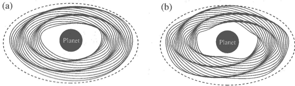
FIGURE 1.17 – Schematic diagrams showing an oblique view of the three-dimensional particle paths that give rise to trailing spiral bending waves near a resonance with an exterior satellite. (a) The two-armed spiral density wave associated with the 3:1 ( m=2 ) inner vertical resonance. (b) The four-armed spiral bending wave associated with the 5:3 ( m=4 ) inner vertical resonances. The pattern rotates with the angular velocity of the satellite and propagates inward from the exact resonance (denoted by the dashed curve). Figure and caption from Murray and Dermott (1999) , p. 493, Figure 10.12.
