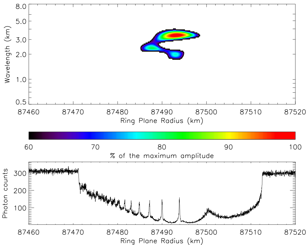
FIGURE 2.32 – WWZ wavelet power profile around Maxwell ringlet, computed from \beta Centauri, rev. 105 individual occultation profile. Though the structure is quite clear and prominent to the eye on the occultation profile, the wwz profile is distorted by the relative importance of the amplitude of the highest wavelengths, hiding smaller amplitudes at the presented scale.
