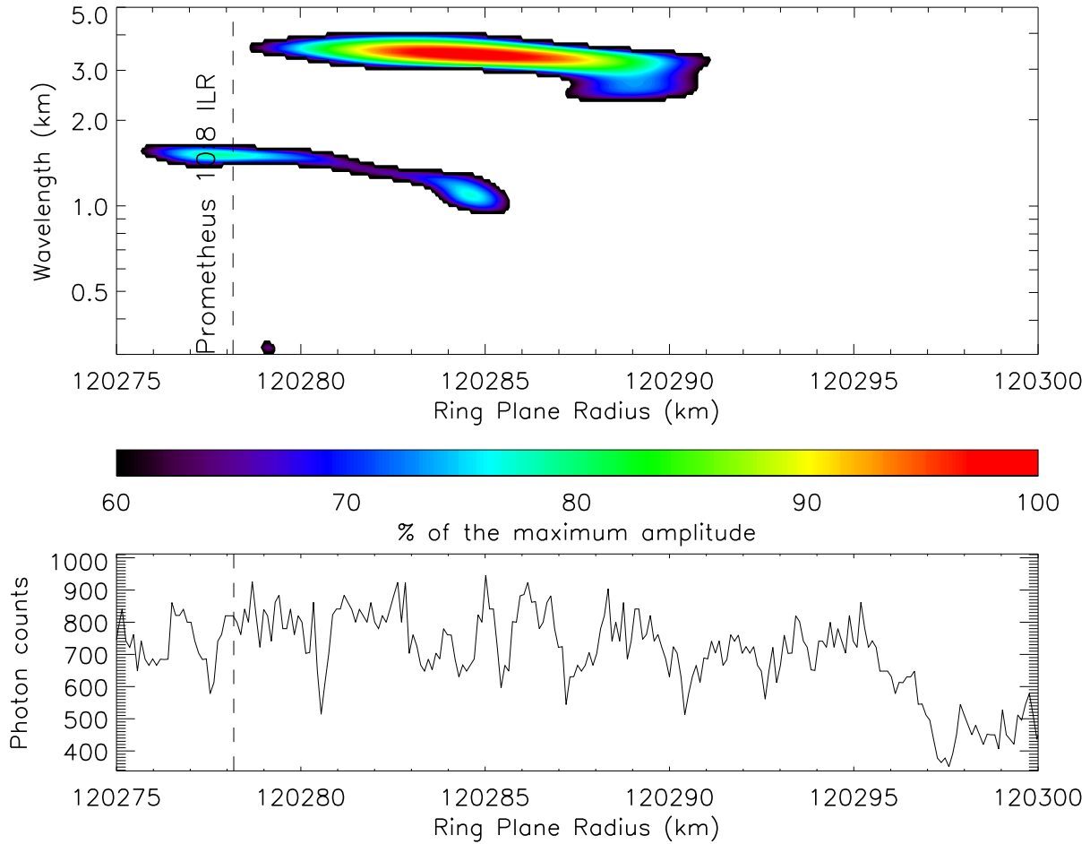
FIGURE 3.13 – WWZ wavelet power profile computed from the \alpha Virginis, rev. 34, occultation of the Promethus 10:8 ILR region. The lower panel shows the photon count rates.
