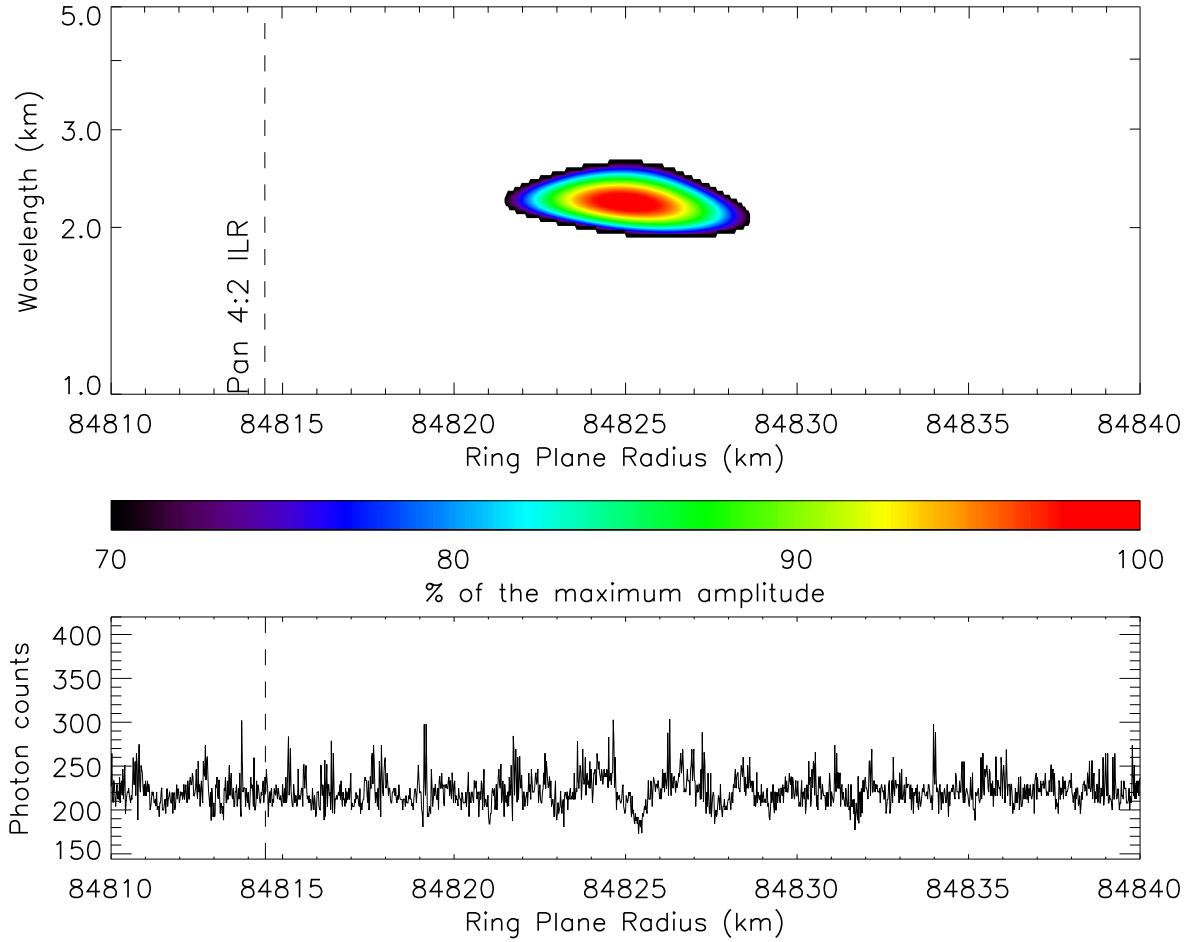
FIGURE 2.13 – WWZ wavelet power profile of feature 20, computed from \beta Centauri, rev. 104 individual occultation profile. Pan 4:2 ILR is at 84814.5 km (vertical dashed line). The relatively long distance between the Pan 4:2 ILR and the wave (about the same distance as the length of the wave itself) together with a very low torque value for this resonance and an inconsistent wave source location from the feature invalidate the possibility of an association. Wave source location is outside the range of this figure, at 84775 \pm 8 km.
