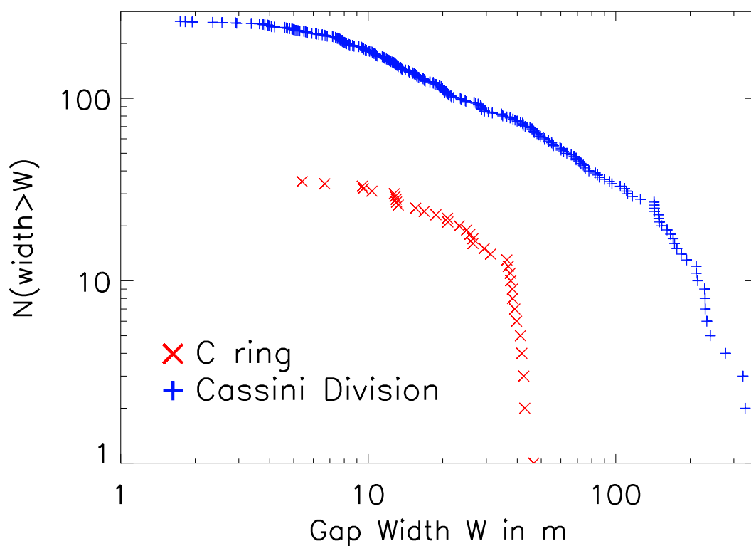
FIGURE 5.20 – Cumulative distribution of the ghosts widths in the C ring and in the Cassini Division. Though figure clarity prevents us from displaying them, we estimate the relative uncertainty on our width measures to be about 1/N , N being the number of points in the ghost.
