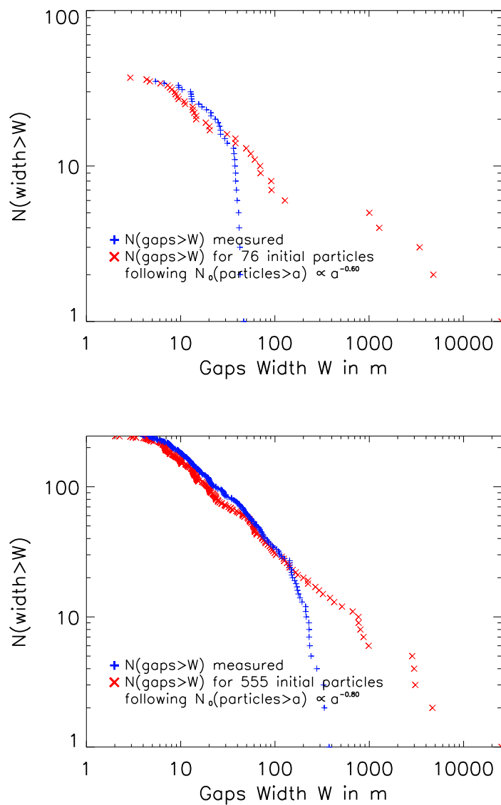
FIGURE 5.21 – Cumulative distribution of the modeled ghosts widths in the C ring (upper panel) and in the Cassini Division (lower panel) for an initial particle size distribution power-law index of 0.6 for the C ring and 0.8 for the Cassini Division. Due to the logarithmic scales, matching the last few scattered points is less important than matching the left part: statistics cannot be applied for such small numbers of the biggest particles.
