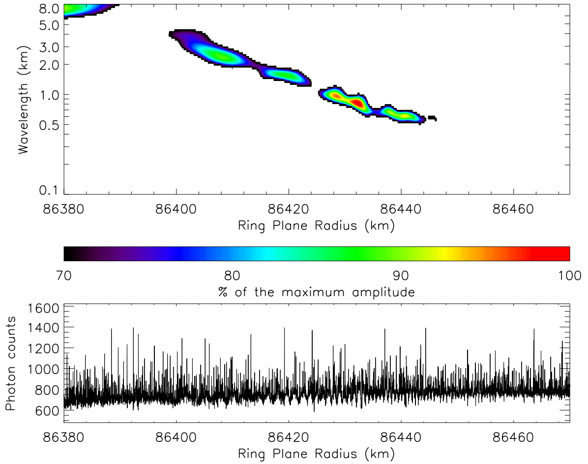
FIGURE 2.22 – Co-added WWZ wavelet power profile of structure 28, computed from individual occultation profiles. Lower panel shows the \beta Centauri, rev. 89 occultation profile. Structure 28 is the most extended feature observed in the C ring, but there is no low order resonance in its vicinity.
