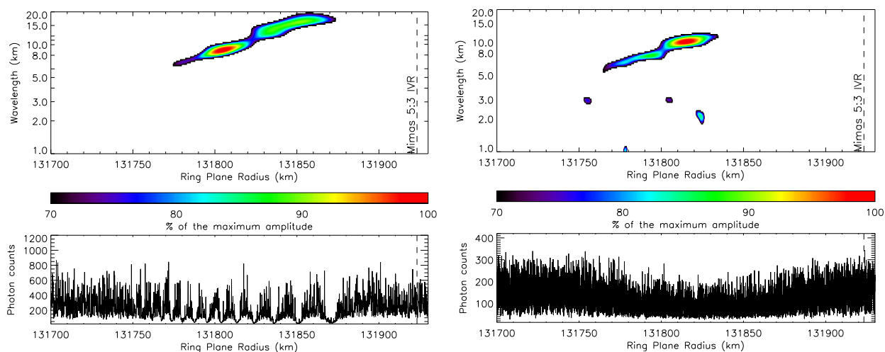
FIGURE 2.3 – WWZ wavelet power profile for the Mimas 5:3 IVR bending wave ( r_V = 131923 km), computed from individual occultation profile of \alpha Virginis, rev. 34 (left) and \beta Centauri, rev. 105 (right).
