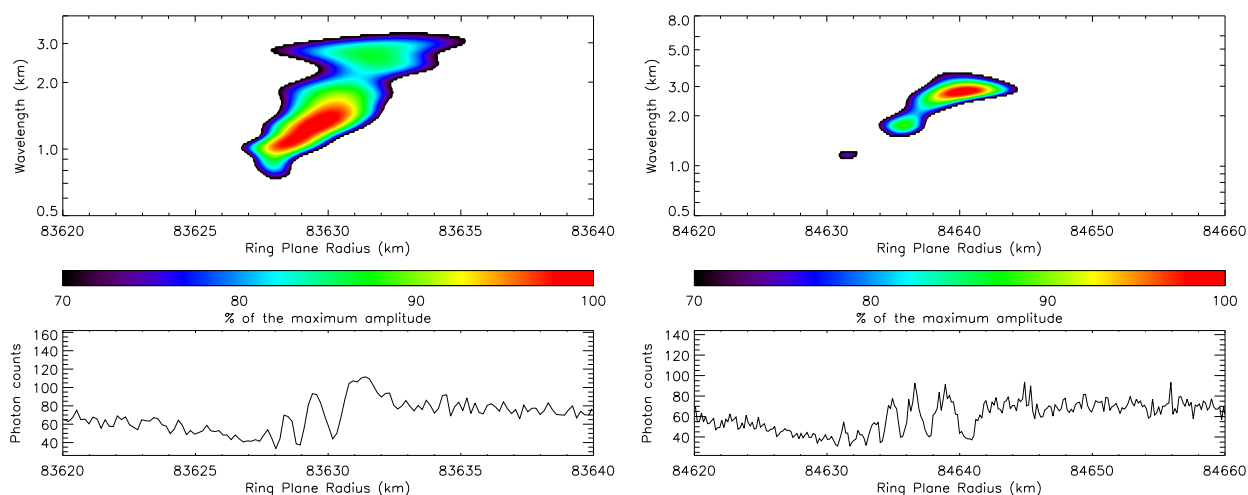
FIGURE 2.27 – WWZ wavelet power profile of structure 18 (left) and 19 (right), computed from individual occultation profile of \zeta Orionis, rev. 47.
