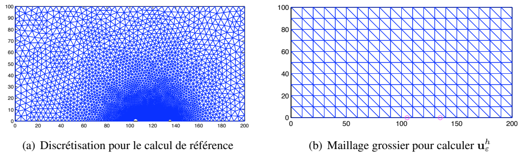
FIGURE 3.9 – Discretisations.
