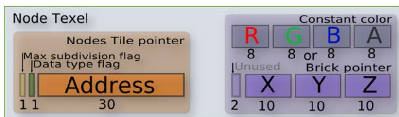
Figure 5.10. Compact octree node encoding into two 32bit values.
