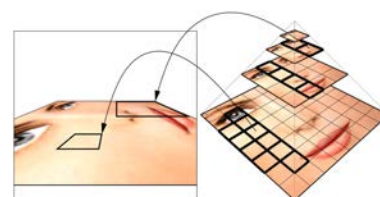
Figure 2.23. Illustration of a tiled MIP-map pyramid representation with correspondence between screen space (left) and texture space (right). Source: [LDN04]
