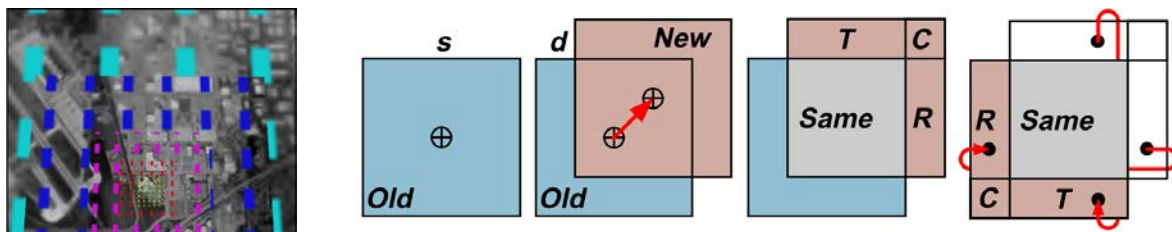
Figure 2.22. Left: Clipmap concentric resolution bands centered on the position of the user. Right: Illustration of the update process inside a clipmap using toroidal addressing. Source: [TMJ98]
