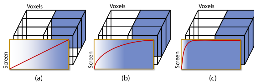
Figure 4.9. Illustration of the result on the screen of volume integration with a lateral per-voxel linear interpolation, with one opaque voxel (a) two correlated opaque voxels (b) and three correlated opaque voxels (c). Correlated cases lead to a non-linear integrated lateral opacity (depicted as a red curve on screens) that diverges from the expected linear result, since (b) and (c) screen results should be the same than (a).
