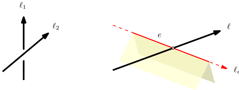
Figure 2: (Left): l_2 passes to the right of l_1 . (Right): In the vicinity of \ell , a line intersects the polytope if and only if it passes to the right of \ell_e .
