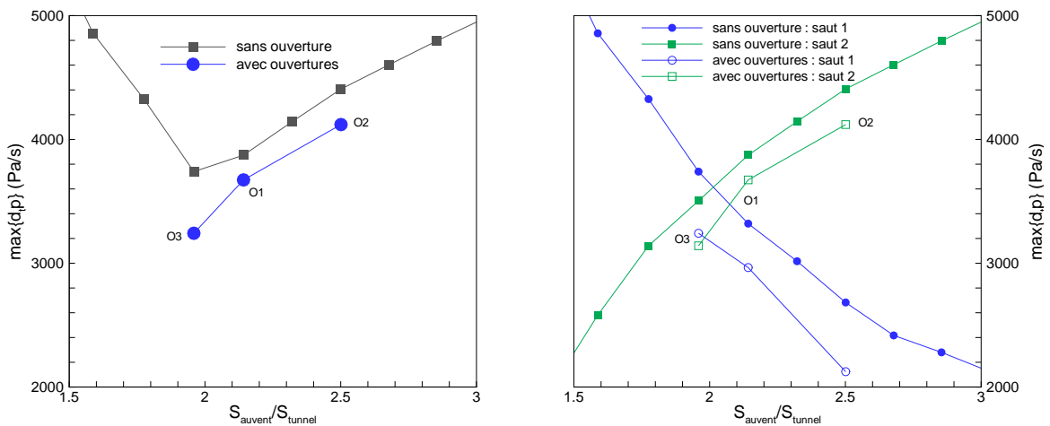
(a) maxima global
