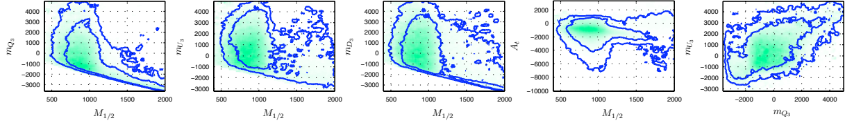
Figure 5.19: Same as Fig. 5.18 but for \epsilon_H = -1 .
