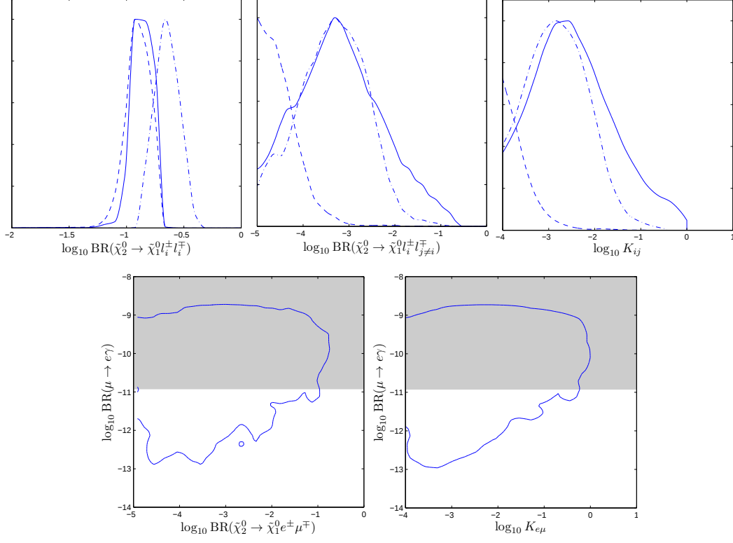
Figure 6.11: Top left: PDF of \text{BR}(\tilde{\chi}_2^0 \rightarrow l_i l_i \tilde{\chi}_1^0) . Plain, dashed and dash-dotted lines correspond to l_i l_i = ee, \mu\mu, \tau\tau respectively. Top center: PDF of \text{BR}(\tilde{\chi}_2^0 \rightarrow l_i l_j \tilde{\chi}_1^0) . Plain, dashed and dash-dotted lines correspond to l_i l_j = e\mu, e\tau, \mu\tau respectively. Top right: Plain, dashed and dash-dotted lines correspond to K_{e\mu}, K_{e\tau}, K_{\mu\tau} respectively. Bottom: 95% BC region of the joint PDF of \text{BR}(\mu \rightarrow e \gamma) with \text{BR}(\tilde{\chi}_2^0 \rightarrow e \mu \tilde{\chi}_1^0) (left) and K_{e\mu} (right).
