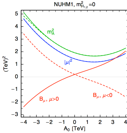
Figure 5.3: Higgs mass parameters in the MSSM with non-universal Higgs masses, for a universal gaugino mass M_{1/2} = 1 TeV, a universal sfermion mass m_0 = 500 GeV, \tan \beta = 10 , and vanishing Higgs soft masses. Note that there is only a “DHMM point” (with meeting |\mu|^2 and B_\mu curves) for \mu > 0 .
