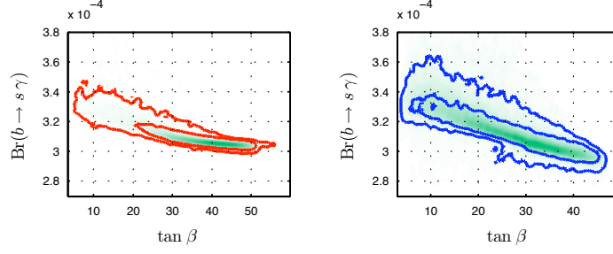
Figure 5.7: Contours of 68% and 95% probability in the \text{BR}(b \rightarrow s\gamma) versus \tan \beta plane, on the left for \epsilon_H = +1 , on the right for \epsilon_H = -1 . The green shading maps the average likelihood per bin, normalized to the maximum likelihood.
