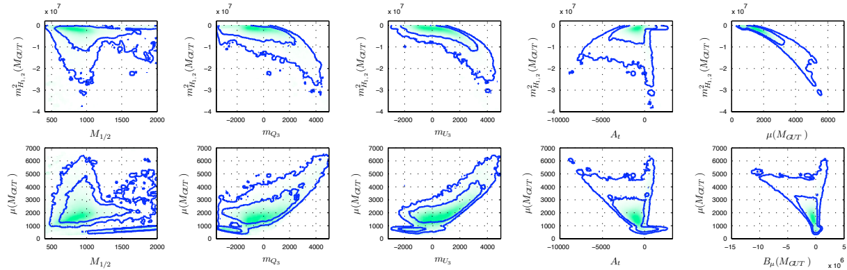
Figure 5.21: Same as Fig. 5.20 but for \epsilon_H = -1 .
