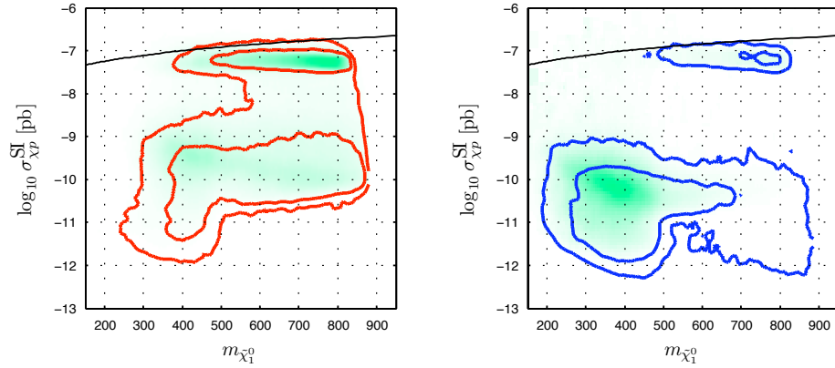
Figure 5.17: Probability distributions in the plane \sigma_{\chi p}^{SI} versus m_{\tilde{\chi}_1^0} for naturalness prior, on the left for \epsilon_H = +1 , on the right for \epsilon_H = -1 . The inner (outer) contours enclose regions of 68% (95%) probability, the green shading maps the average likelihood, and the black lines show the limit from CDMS-II, which is currently providing the strongest bound in this mass range.
