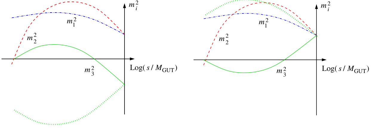
Figure 4.1: Qualitative RG evolution of m_1^2 (blue dot-dashed curve), m_2^2 (red dashed curve), and m_3^2 (green solid curve) as a function of the scale s , between s = M_{\text{EWSB}} and s = M_{\text{GUT}} . A_t at the GUT scale is sizeable and positive. The green dotted curve is m_3^2 for the wrong \text{sign}(\mu) , which does not lead to realistic EWSB. Left panel: \epsilon_H = -1 requires \text{sign}(\mu) = -1 . Right panel: \epsilon_H = +1 requires \text{sign}(\mu) = +1 .
