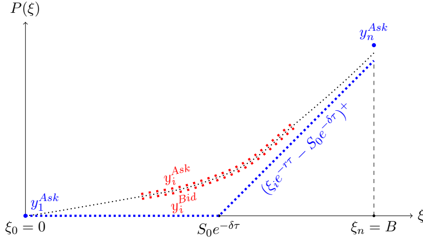
Figure 7.2: This graph sums up the set of constraints verified by estimated put prices, which are solutions of the quadratic optimization problem described in eq. (P1). Estimated put prices m_1, \dots, m_n on the “dense” grid \xi_1, \dots, \xi_n are displayed as black dots. They must lie in-between the bid-ask quotes, which are represented by thick red dots ranging over quoted strikes \xi_{i_1}, \dots, \xi_{i_s} , which correspond to a sparse subset of the underlying dense grid \xi_1, \dots, \xi_n . In addition, extreme put prices m_1 and m_n are bounded above by y_1^{Ask} = 0 and y_n^{Ask} , respectively, where the value of y_n^{Ask} is given in Section 7.7.3. Both y_1^{Ask} and y_n^{Ask} appear as thick blue dots at strikes \xi_1 = 0 and \xi_n = B , respectively. m_1, \dots, m_n must also verify the in-sample constraints described by the lhs of eq. (7.27). In particular, the lhs of eq. (7.27) ensures that the m_i s are lower-bounded by the (\xi_i e^{-r\tau} - S_0 e^{-\delta\tau})^+ s, which appear as thick blue dots. Since this lower-bound is worth 0 for i = 1 , this, together with the upper-bound y_1^{Ask} = 0 actually impose m_1 = 0 . Finally, m_1, \dots, m_n verify both eq. (7.28) and eq. (7.29) above. The latter constraint imposes in-sample convexity.
