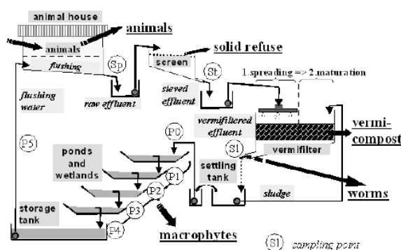
FIGURE 1. General scheme of the prototype of clean piggery built at Guernévez, with indication of the sampling points (in the circles).
