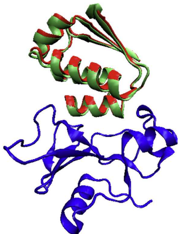
Fig. 1. Comparison of the energy-minimized (green) and experimental (red) positions of barstar in the barnase/barstar complex. Barnase is plotted in blue. The C_{\alpha} rmsd between the experimental and calculated position is 0.69 \text{ \AA} . The molecular graphics were prepared using VMD. 60
