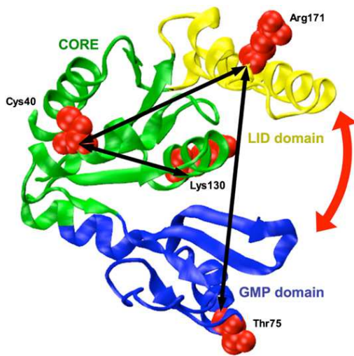
FIGURE 1 A cartoon representation of GK with the pulling directions tested experimentally by Tseng et al. (48). The color coding of the protein is according to the domain definitions of Hible et al. (67). The GMP and ATP binding sites are located at the GMP/CORE and CORE/LID interfaces, respectively. The arrow indicates the direction of the opening/closing transition, which constitutes the first mode of motion of the protein. The images in this figure and in the upper part of Fig. 5 were prepared using visual molecular dynamics (71).
