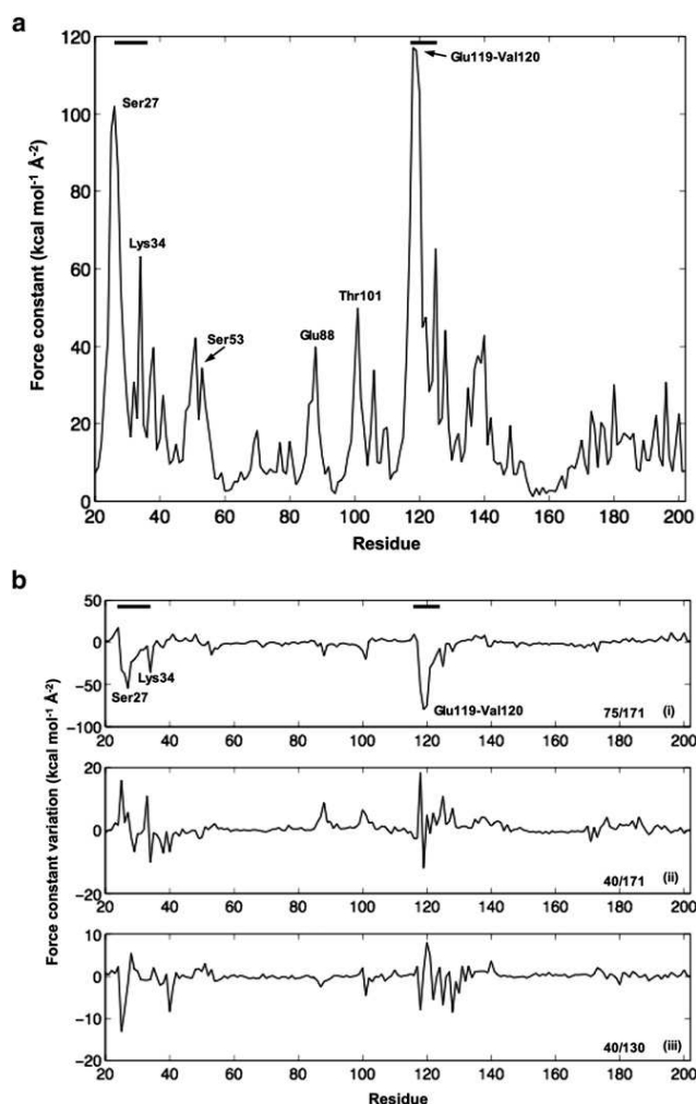
FIGURE 2 (a) Rigidity profile of GK when no mechanical stress is applied on the protein. (b) Variation of the force-constant profile upon applying an external constraint on the protein in pulling directions 75/171 (upper), 40/171 (middle), and 40/130 (lower). The black horizontal bars at the upper left of Fig. 2, a and b , indicate the position of the P-loop and the \beta 7-sheet along the sequence.
