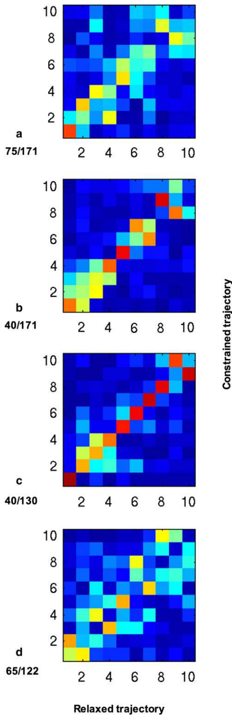
FIGURE 3 Inner-product matrices of the 10 first eigenvectors of the constrained trajectories over the relaxed trajectory. The pulling directions are (a) 75/171, (b) 40/171, (c) 40/130, and (d) 65/122. The color scale ranges from 0 to 1.
