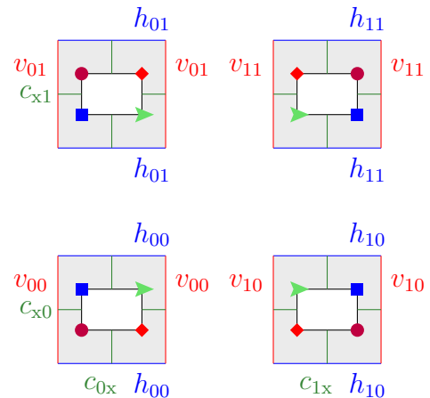
Figure 4: Homology generators for X(a, b) .
