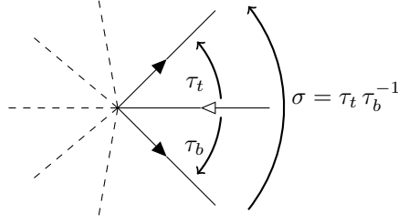
Figure 4.2: The relation \sigma = \tau_t \tau_b^{-1} on the level of the interval diagram of \pi .
