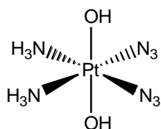
cis, trans, cis -[Pt(N 3 ) 2 (OH) 2 (NH 3 ) 2 ]
