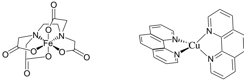
Figure 28. Structures des complexes [\text{Fe}^{\text{II/III}}(\text{EDTA})]^{2-} et [\text{Cu}^{\text{I/II}}(\text{phen})_2]^{+2+} .
