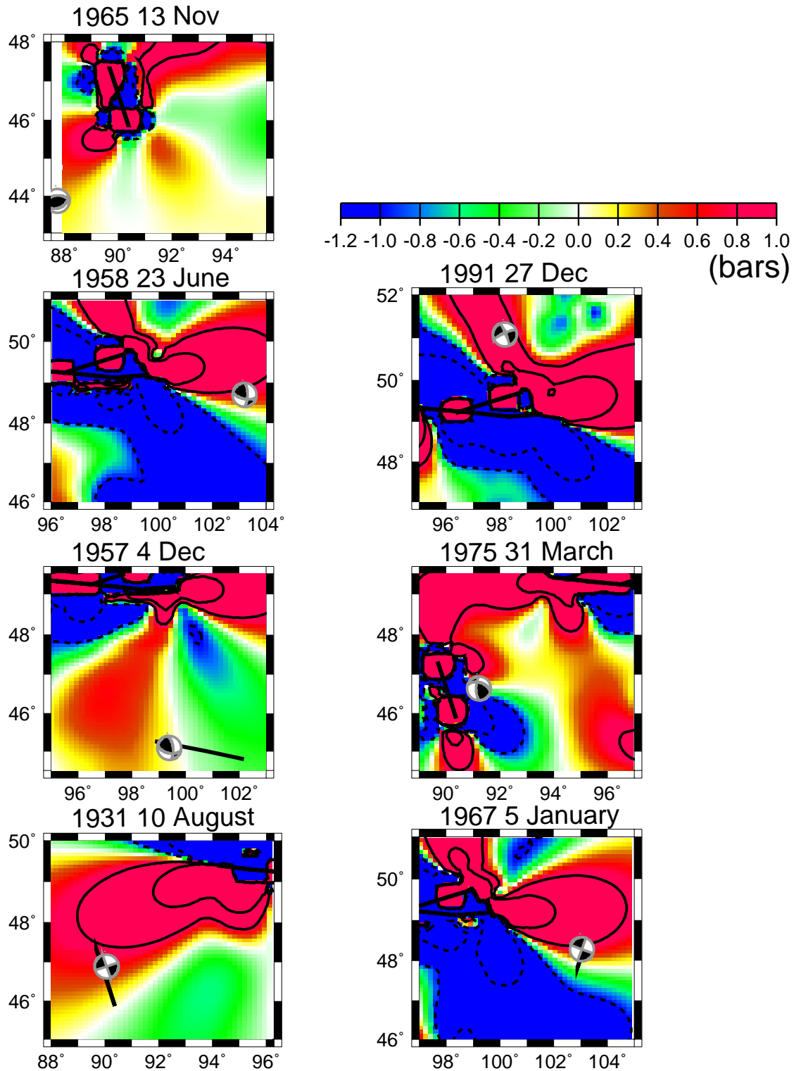
FIG. 4.12: Cumulative static plus viscoelastic stress change evaluated on Model A (weak mantle, weak crust) just prior to the occurrence of each of the non-Baikal secondary earthquakes listed in table 4.1. Other conventions as in figure 4.10.
