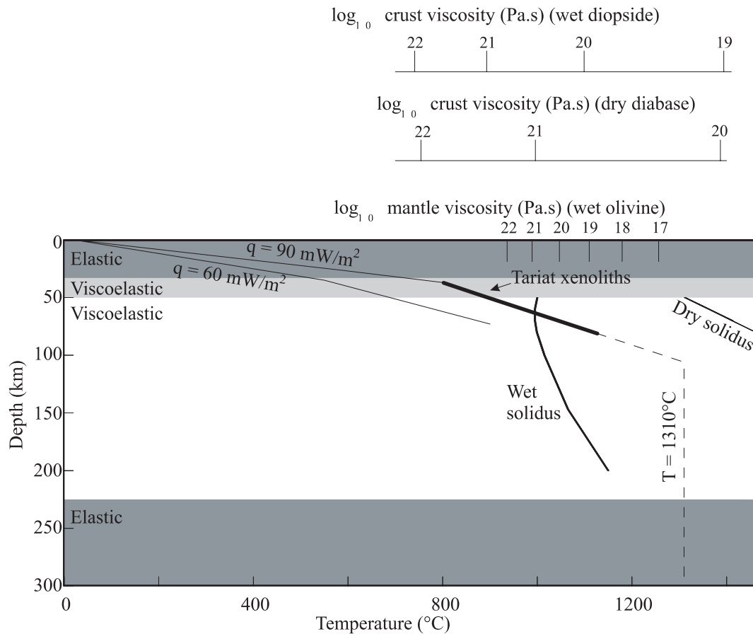
FIG. 3.9: Viscoelastic stratification used to model postseismic deformation in Western Mongolia. The thick black line represents the geotherm for the Tariat region (Ionov et al., 1998), the thin black lines are theoretical conductive geotherms for continental domains for surface heat flows of 60 and 90 \text{mW/m}^2 (Pollack et Chapman, 1977). The experimentally-derived viscosity law for wet olivine are from Hirth et Kohlstedt (1996), for dry diabase and wet diopside from Mackwell et al. (1998). These laws are computed with \dot{\epsilon} constant ( \dot{\epsilon} = 2,2 \times 10^{-15} \text{ s}^{-1} ) for the crust and \sigma constant ( \sigma = 0,3 \text{ MPa/yr} ) for the mantle.
