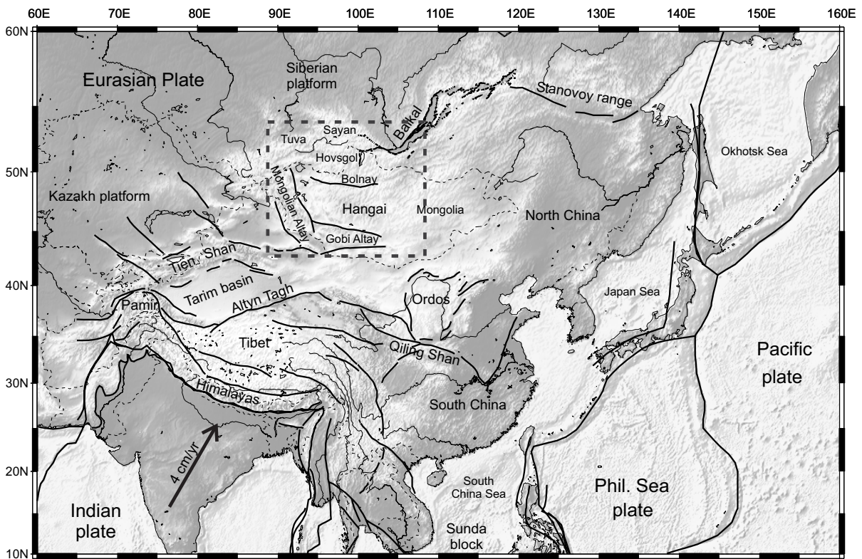
FIG. 2.1: Topography, main active faults, and index of the geographical names used in this paper. The box centered on Mongolia shows the study area, shown in more detail on figure 2.2.
