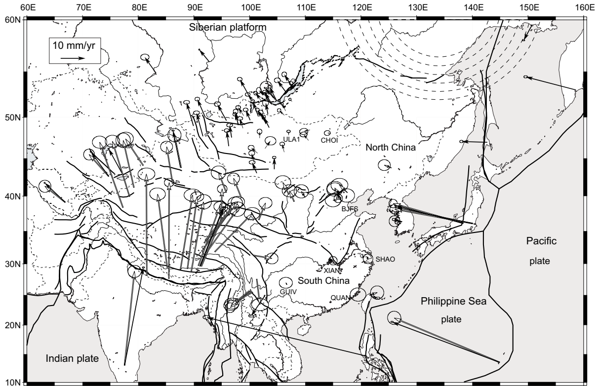
FIG. 2.9: GPS-derived velocities with respect to East China. Black arrows : our solution ; Grey arrows : Wang et al. (2001)'s solution after transformation into ITRF2000 and rotation into a Eurasia-fixed frame (explanation in text). Ellipses are 95% confidence. Dashed lines are small circles around the rotation pole of East China with respect to Eurasia.
