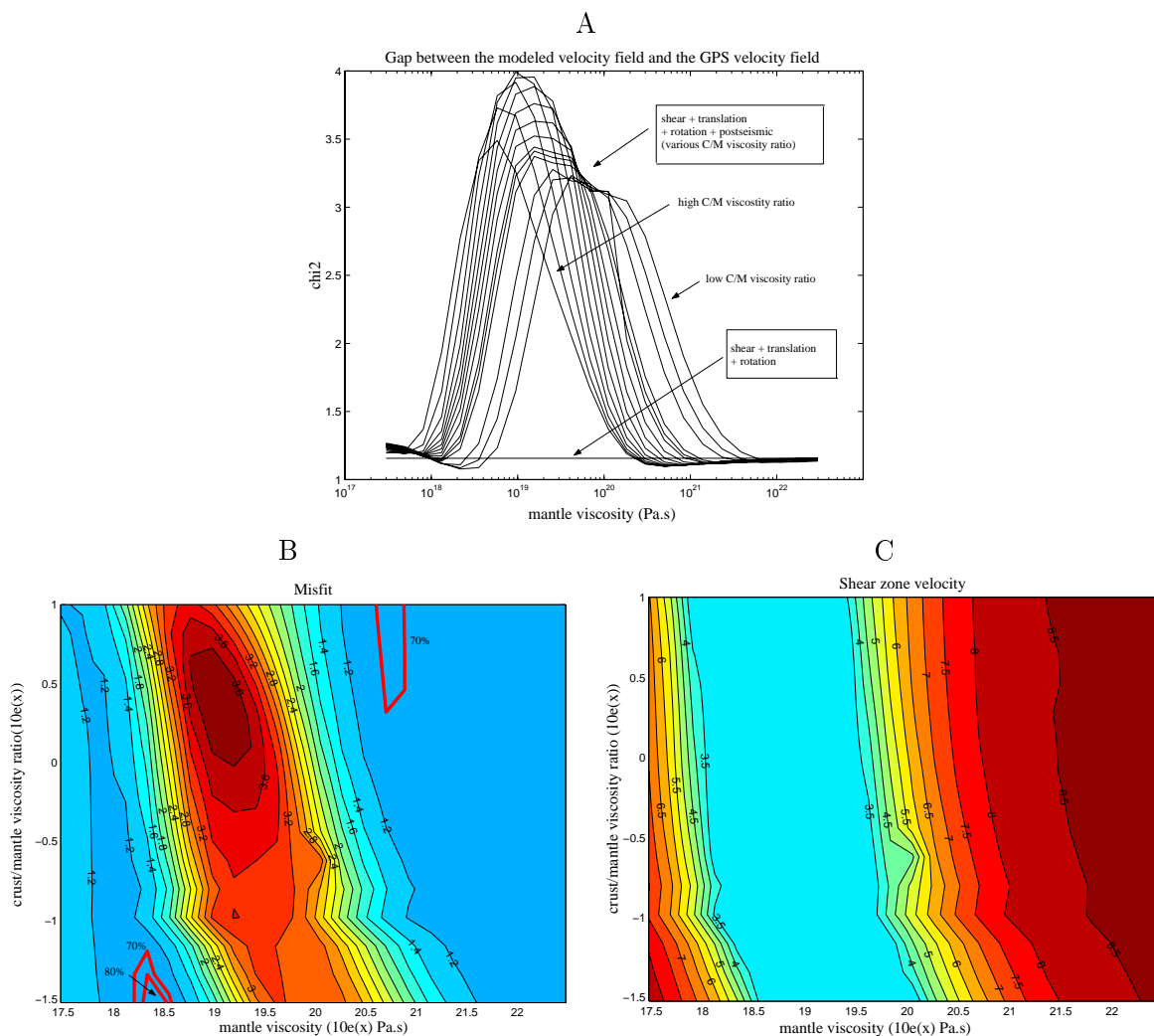
FIG. 3.10: Result for the inversion of the Mongolia GPS data set (29 stations), with a covariance matrix derived from the formal GPS errors with the restriction that the standard deviation in any velocity component must be greater than 1 mm/yr and with “Vsz restricted” scheme. A : \chi^2 as a function of upper mantle viscosity with postseismic effects (curves), without postseismic effects (horizontal line). B : Logarithmic misfit of GPS data with respect to the viscoelastic relaxation model as a function of mantle viscosity and crust-to-mantle viscosity ratio. The contours show the 70% and 80% confidence area where the null hypothesis is verified by an F-test (i.e., accounting for postseismic effects significantly improves the \chi^2 ). C : Shear velocities across Mongolia obtained from this inversion (in mm/yr).
