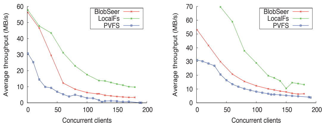
(a) Upload average throughput for 30 Cumulus servers.
