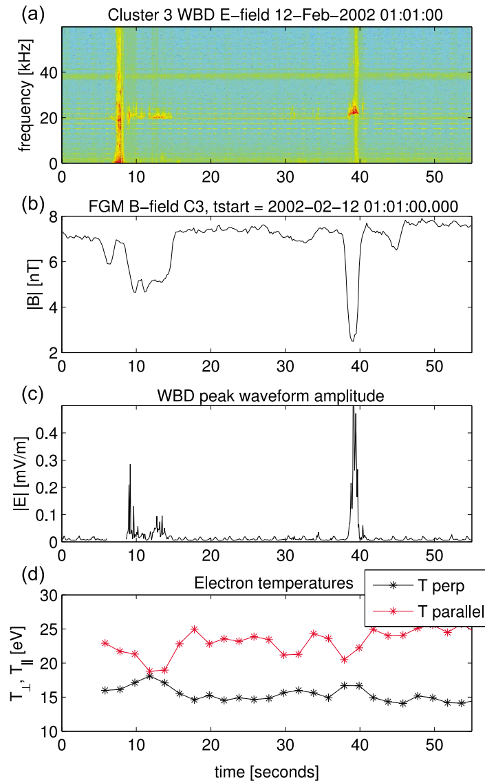
Figure 7. Detailed view of magnetic holes observed by Cluster. (a) Electric field spectrogram (WBD instrument). The strong broadband signature just before the first hole is an instrumental effect (a signature of Whisper resonance sounder sweep). (b) Magnetic field magnitude (FGM). (c) Peak electric field amplitude (WBD). (d) Parallel and perpendicular electron temperature.
