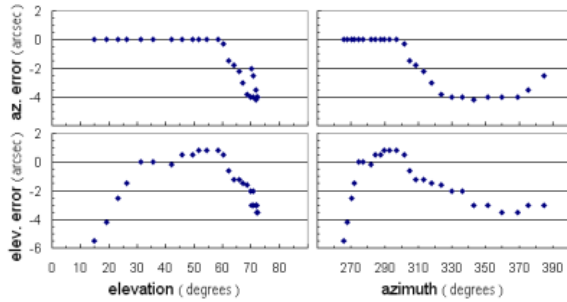
Fig. 5. Observed absolute tracking error for a star with |\delta| = -3^{\circ}42' . Same experimental setup as described in Fig. 4, with the displacement measured at regular intervals.
