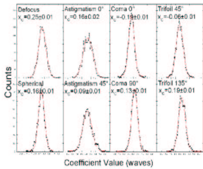
Fig. 4. Zernike coefficients histograms from 75 PPDS restorations.
