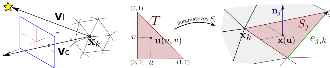
Figure V.2: Notations. Parametrization of the discrete representation of the surface into a triangle mesh.
