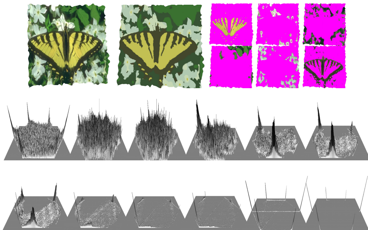
Figure IV.8: Segmentation results and histogram evolution of the convex variable onto a graph representation of the convex set K (a standard 6-simplex here). The six nodes of the graph corresponds to the six values of the mean colors of each region.
