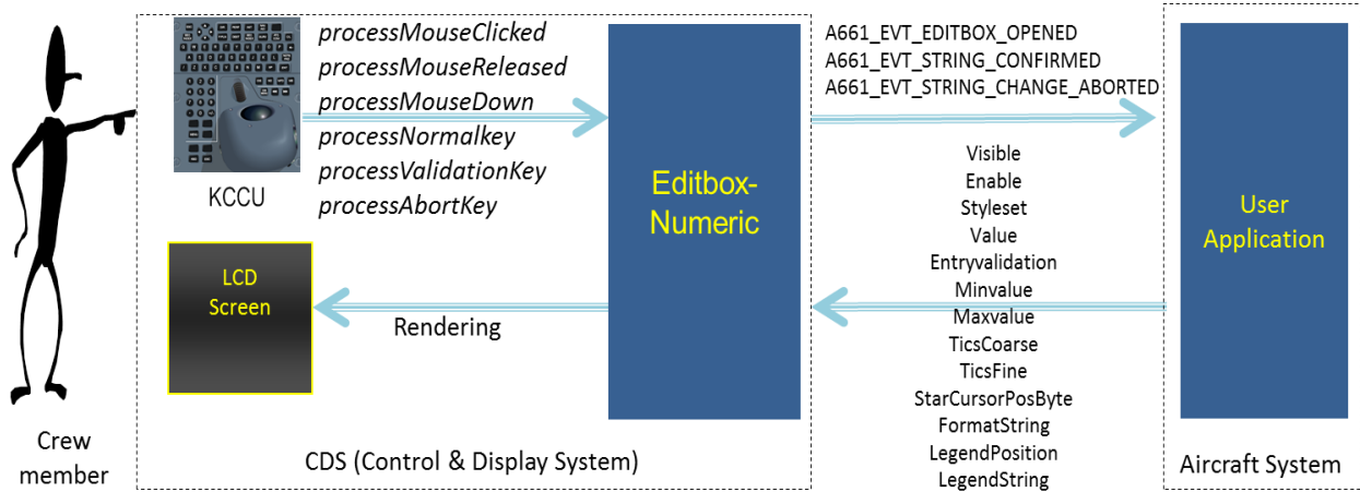
Figure IV.20 Interface EditBoxNumeric
