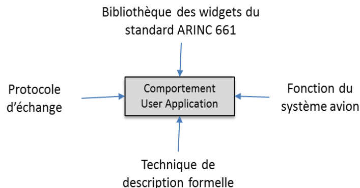
Figure III.16 Spécification UA
