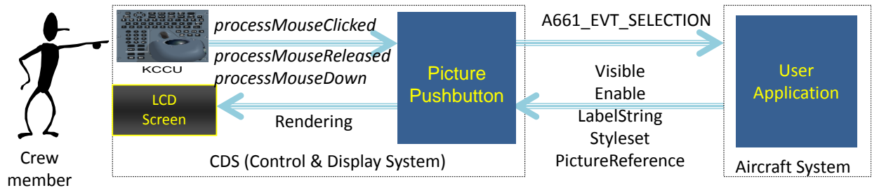
Figure IV.8 Interface PicturePushButton
