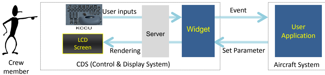
Figure IV.6 Architecture de communication widget et UA
