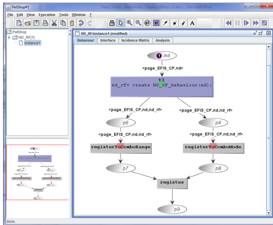
Figure II.27 Environnement PetShop
