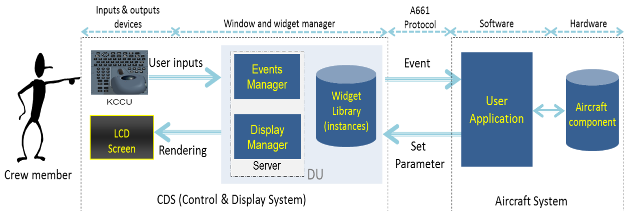
Figure III.3 Architecture de communication ARINC 661 DU/UA
