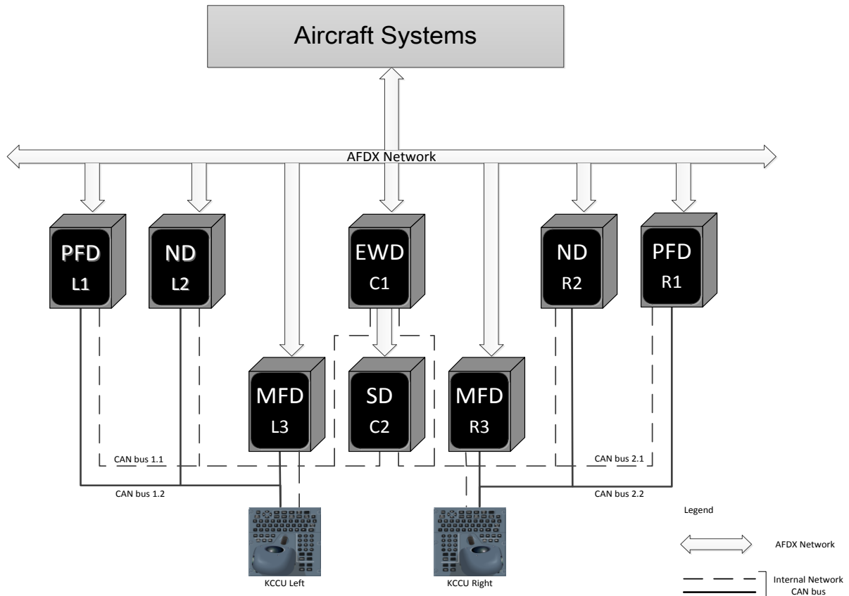
Figure III.6 Architecture matérielle du CDS A380
