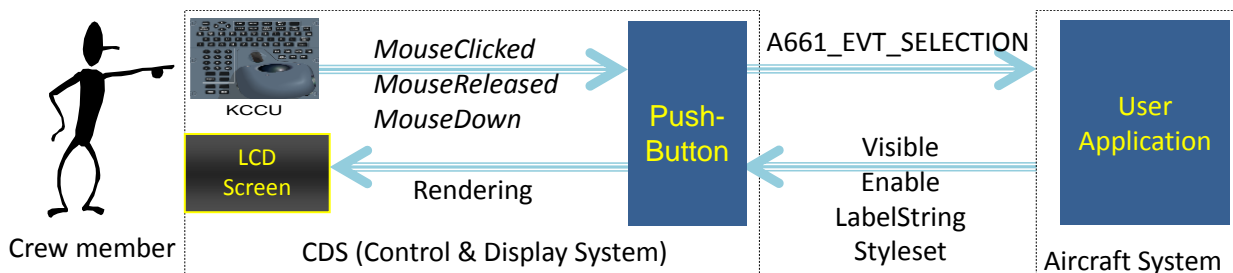
Figure III.14 Communication sur le Pushbutton
