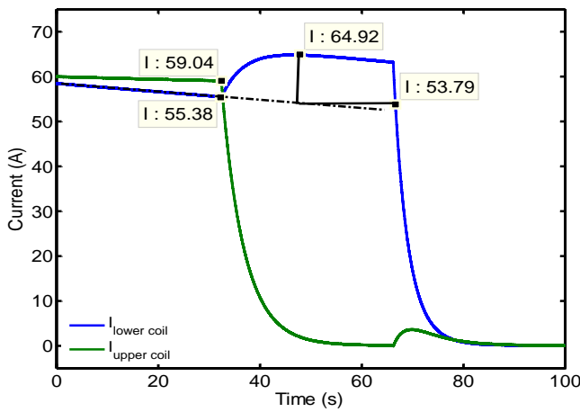
Figure 4-51: Sequential discharge
