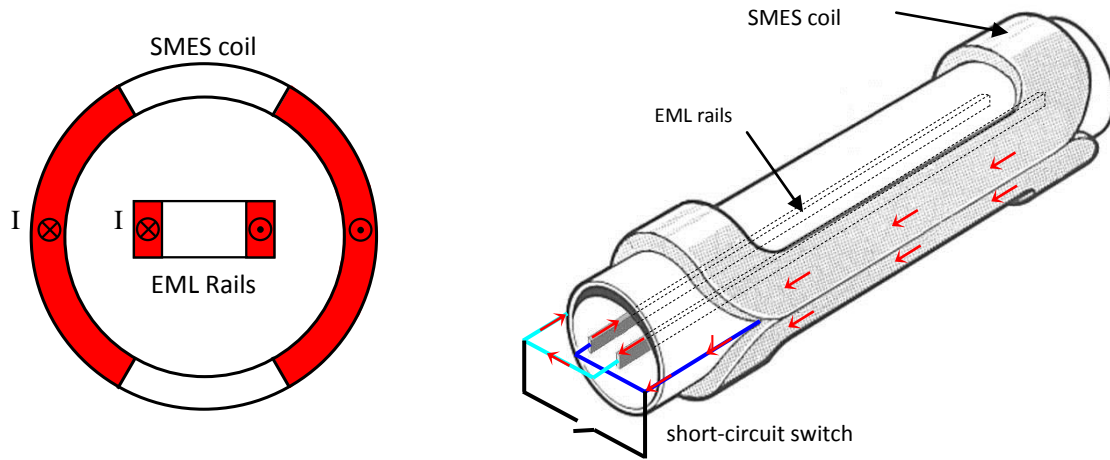
Figure 2-19: Possible SMES-launcher integration for S 3 EL concept with dipole-type coil. Cross section (left) and perspective view (right)
