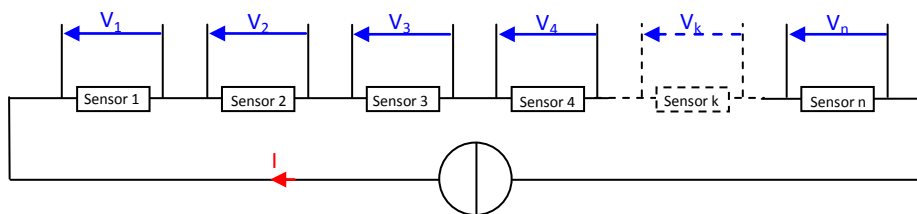
Figure 4-5: Multiple sensor 4 wires measurement
