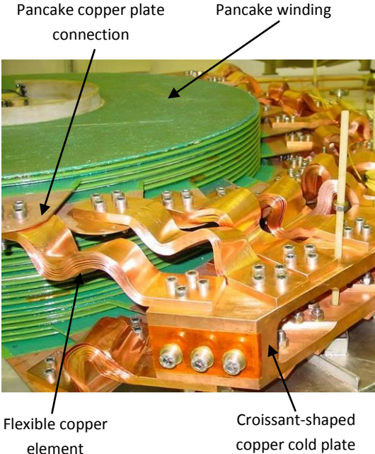
Figure 3-4 : Pancake stack and cooling plates
