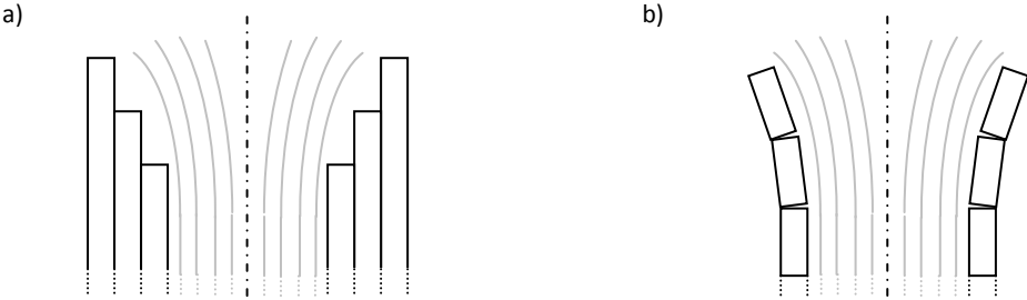
Figure 1-18: Optimized solenoid ends
