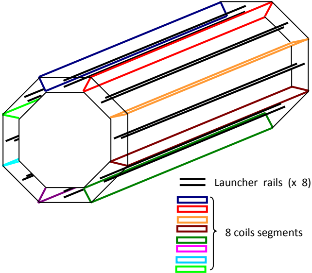
Figure 2-27: S 3 EL variant with several coupled launchers
