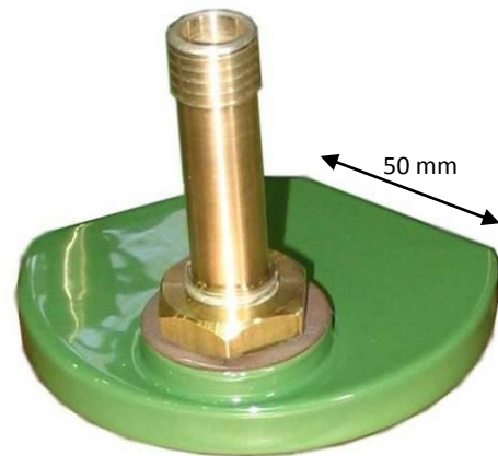
Figure 4-12: Current lead segment
