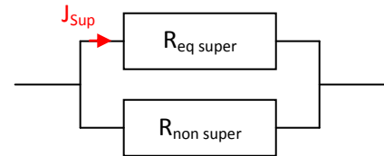
Figure 1-7: Equivalent resistance of an HTS conductor
