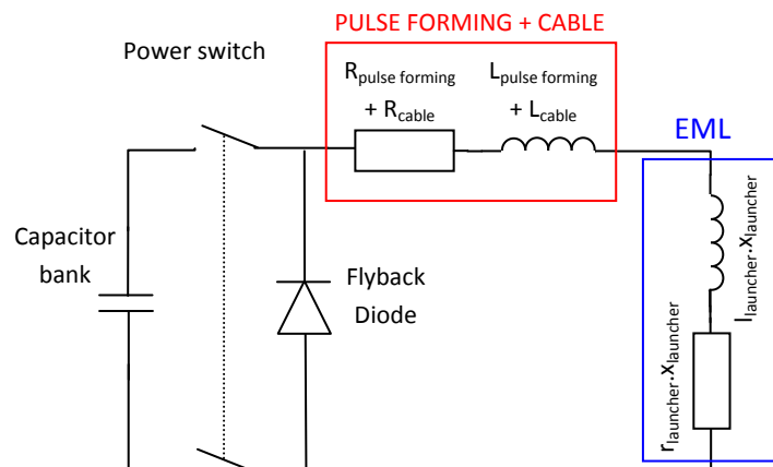
Figure 2-5: Capacitor powering circuit for EML
