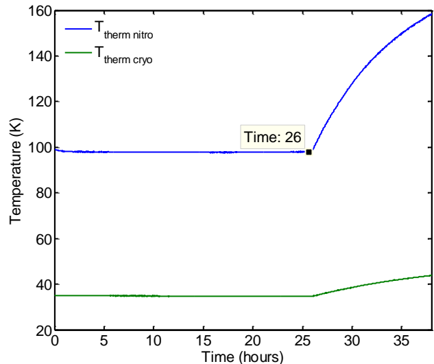
Figure 4-35: Nitrogen tank cooling capacity (graph starts immediately after refilling)
