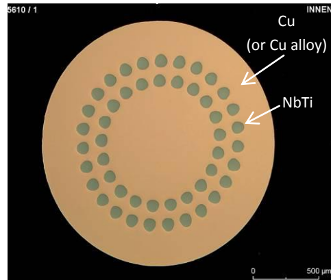
Figure 1-19: Typical LTS cable cross section (NbTi with copper matrix) by Bruker
