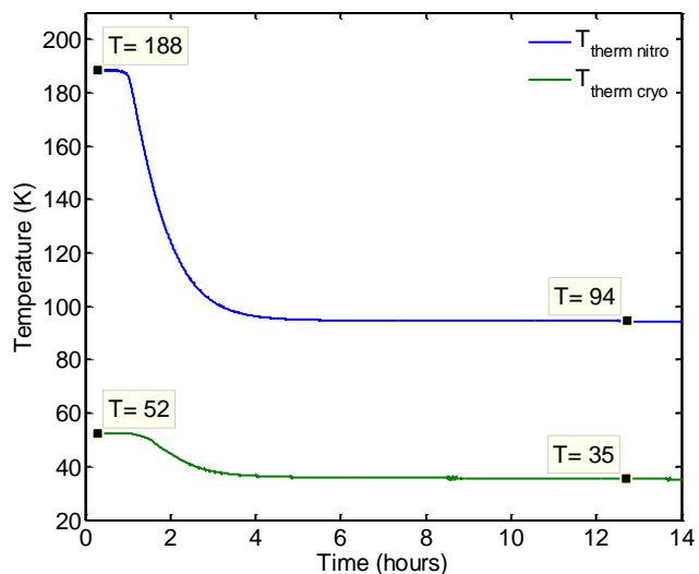
Figure 4-34: Nitrogen cooling
