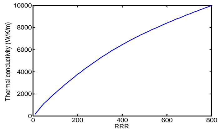
Figure 4-10: Interpolated values for thermal conductivity of copper vs. RRR at 15 K
