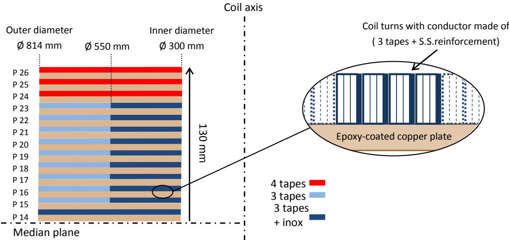
Figure 3-3 : Conductor types in SMES I lower-half coil (upper-half is symmetrical)
