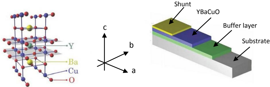
Figure 1-4 : Comparison between crystalline structure (left) and tape orientation (right) for YBCO superconductor.
