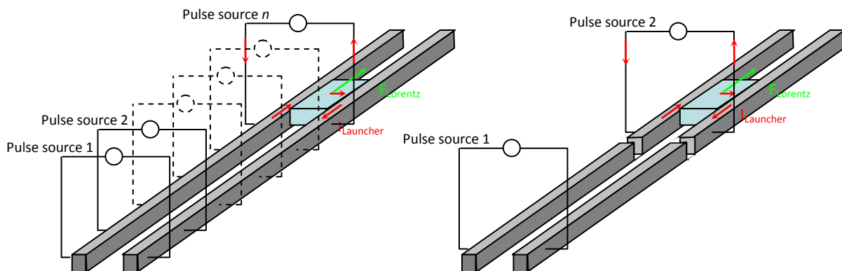
Figure 2-2 : Distributed powering concept (left) and segmented launcher concept (right)
