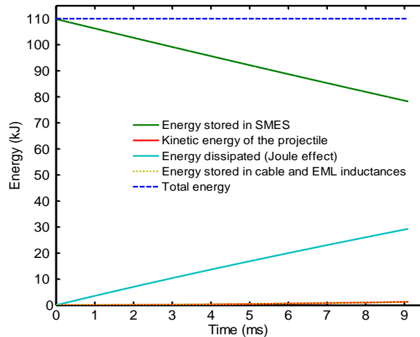
Figure 2-11 : Energy transfer during 110 kJ SMES-powered launch at 400 m/s
