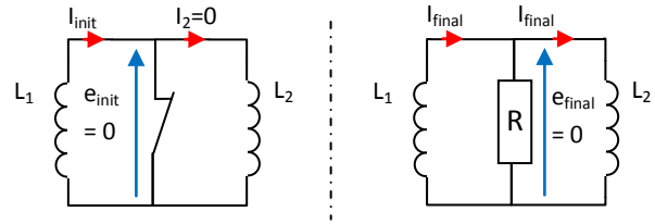
Figure A-1: Initial (left) and final (right) states of constant inductance - inductance discharge
