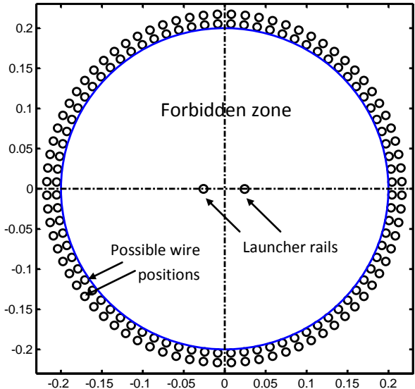
Figure 2-23: Simulated geometry
