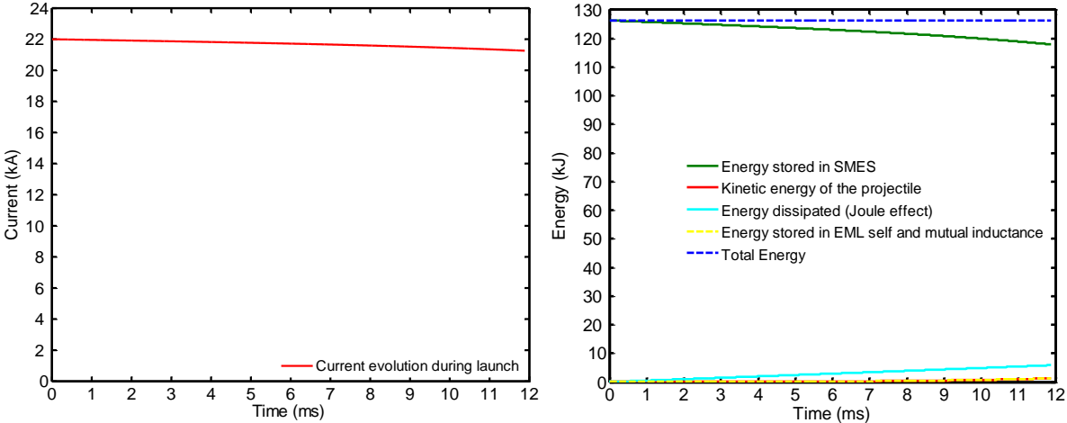
Figure 2-25 : Current (left) and Energy (right) evolution for optimized S^3\text{EL} configuration (output speed 400 m/s)
