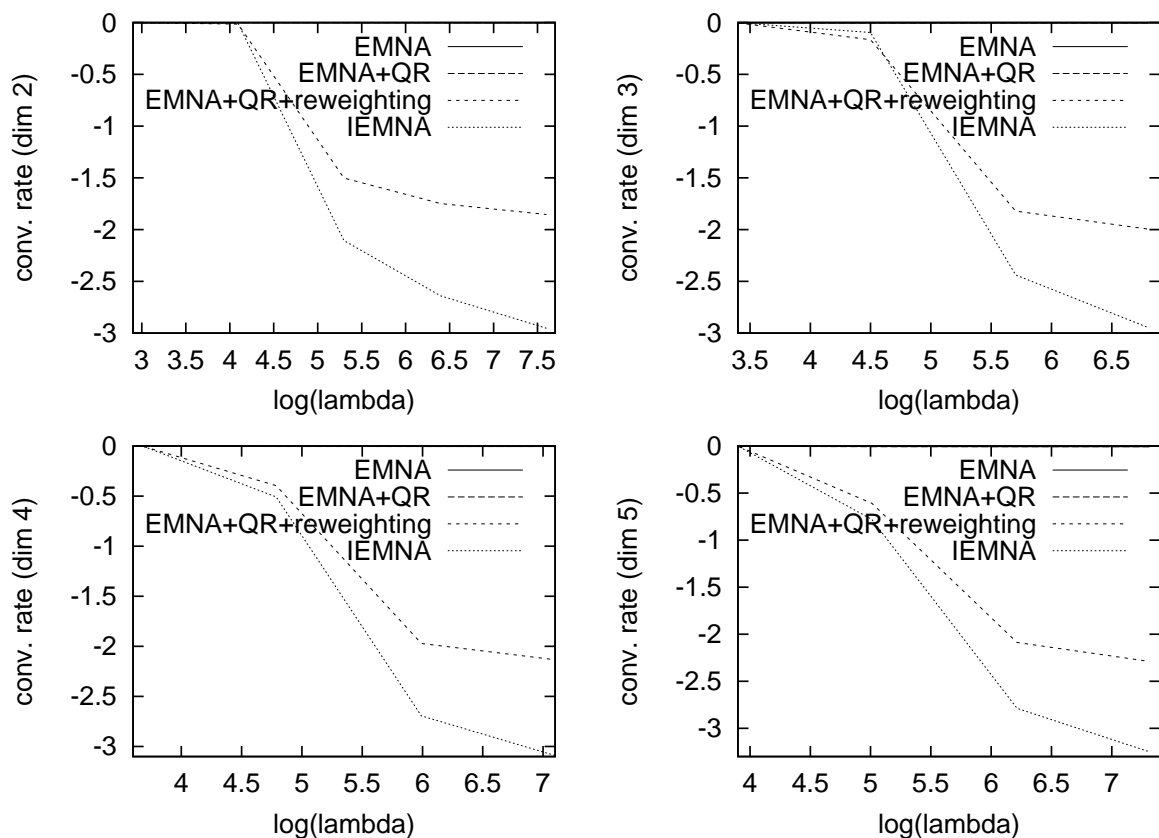
Figure 2.24: Results on the Sphere function. Convergence rates for EMNA, EMNA+QR, EMNA+QR+reweighting, and IEMNA=EMNA+QR+LB+reweighting, with very small initial step size. The smaller, the better the result. EMNA, EMNA+QR have convergence rate nearly 0. The main important tool here is reweighting, but IEMNA still improves the results over EMNA+QR+reweighting.
