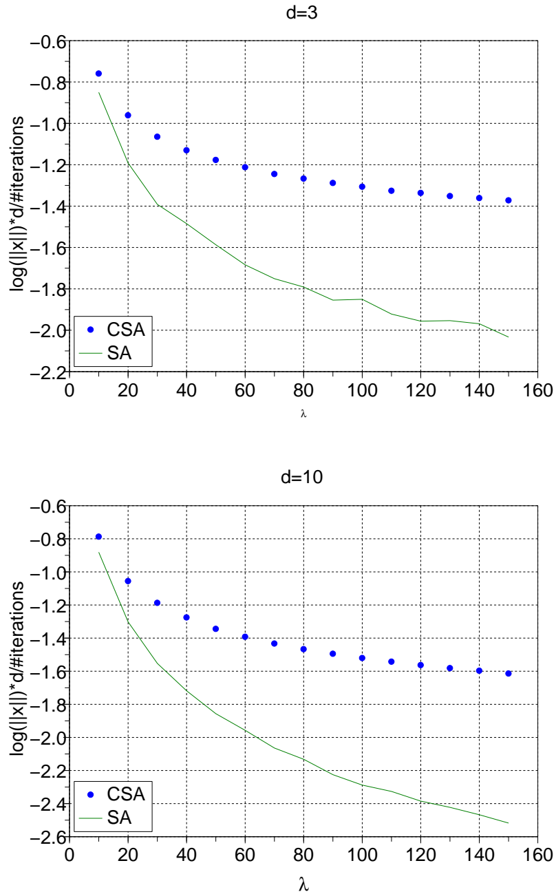
Figure 2.9: Results for \mu = 1 on the Sphere function in dimensions 3 (Top) and 10 (Bottom). SSA is not presented as it does not make sense for \mu = 1 . As shown by this figure (compared to \mu = \frac{1}{4} and \mu = \frac{1}{2} ), \mu = 1 is quite weak for large dimension and the absence of SSA version for that case is therefore not a trouble.
