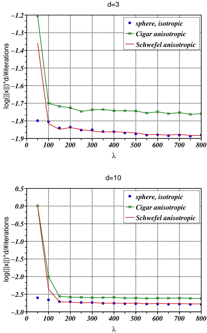
Figure 2.11: Results of the anisotropic version of the SSA algorithm in dimensions 3 (Top) and 10 (Bottom).
