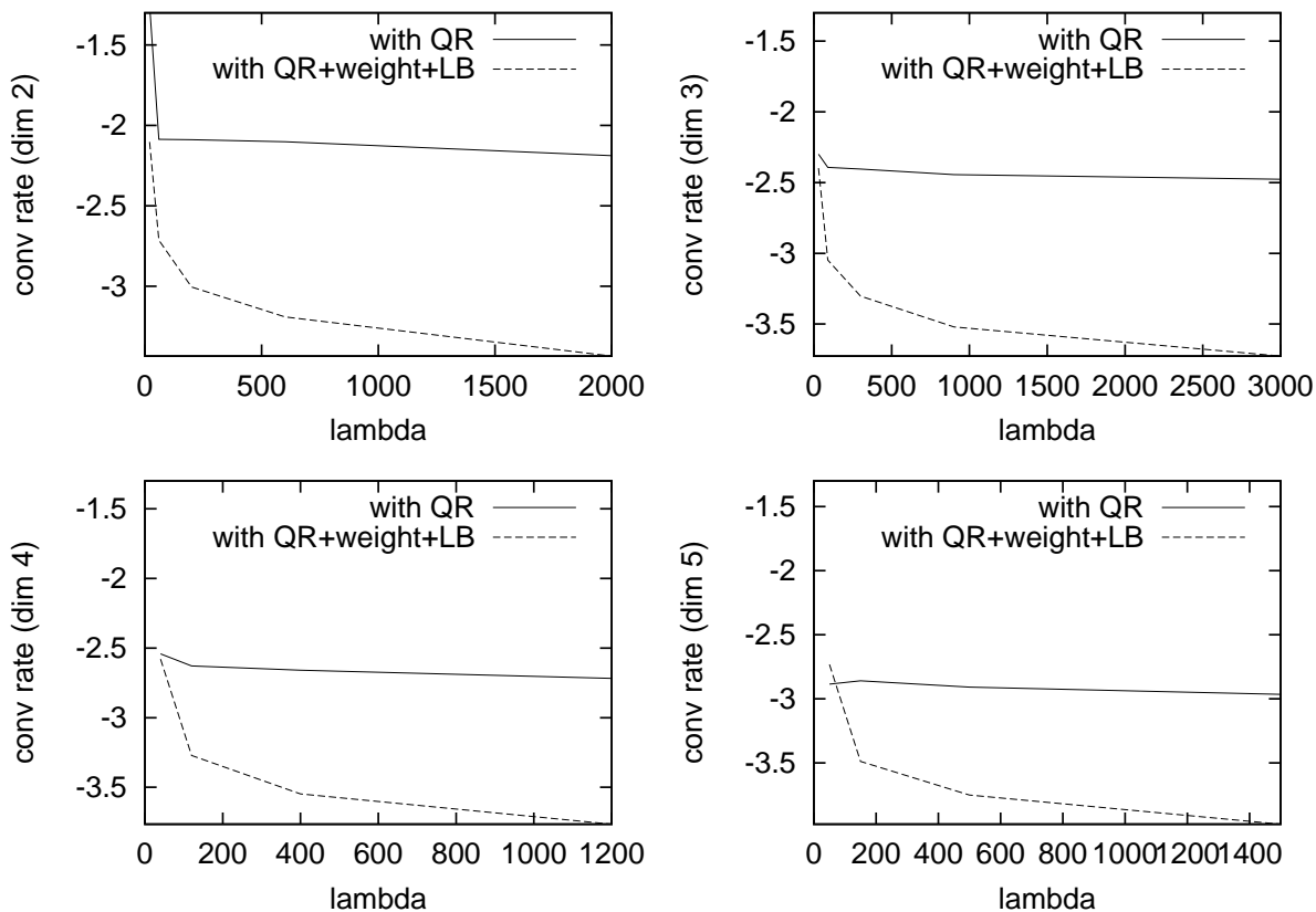
Figure 2.22: Synthesis of the performance of LB in the case of the Sphere. Convergence rate of EMNA with QR mutations (as in [Teytaud and Gelly, 2007, Teytaud, 2008b]), which provide the state of the art convergence rates for EMNA with \lambda large before this work, and convergence rates of IEMNA=EMNA+QR + reweighting + LB (Algorithm 7). The improvement is very clear for \lambda large. This is not in the case with poor initialization; with poor initialization (see text), results are much more impressive for reweighting (which avoids premature convergence, as shown in [Teytaud and Teytaud, 2009c]), but in that case LB would be harmful (LB makes it more difficult to recover from the bad initialization).
