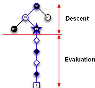
Figure 5.2: Illustration of the Monte-Carlo Tree Search algorithm. The Descent part consists in choosing a new node according to a bandit formula. The evaluation policy appears when we reach a situation outside the Tree. In the simplest case, the evaluation is done by doing a Monte-Carlo simulation.
