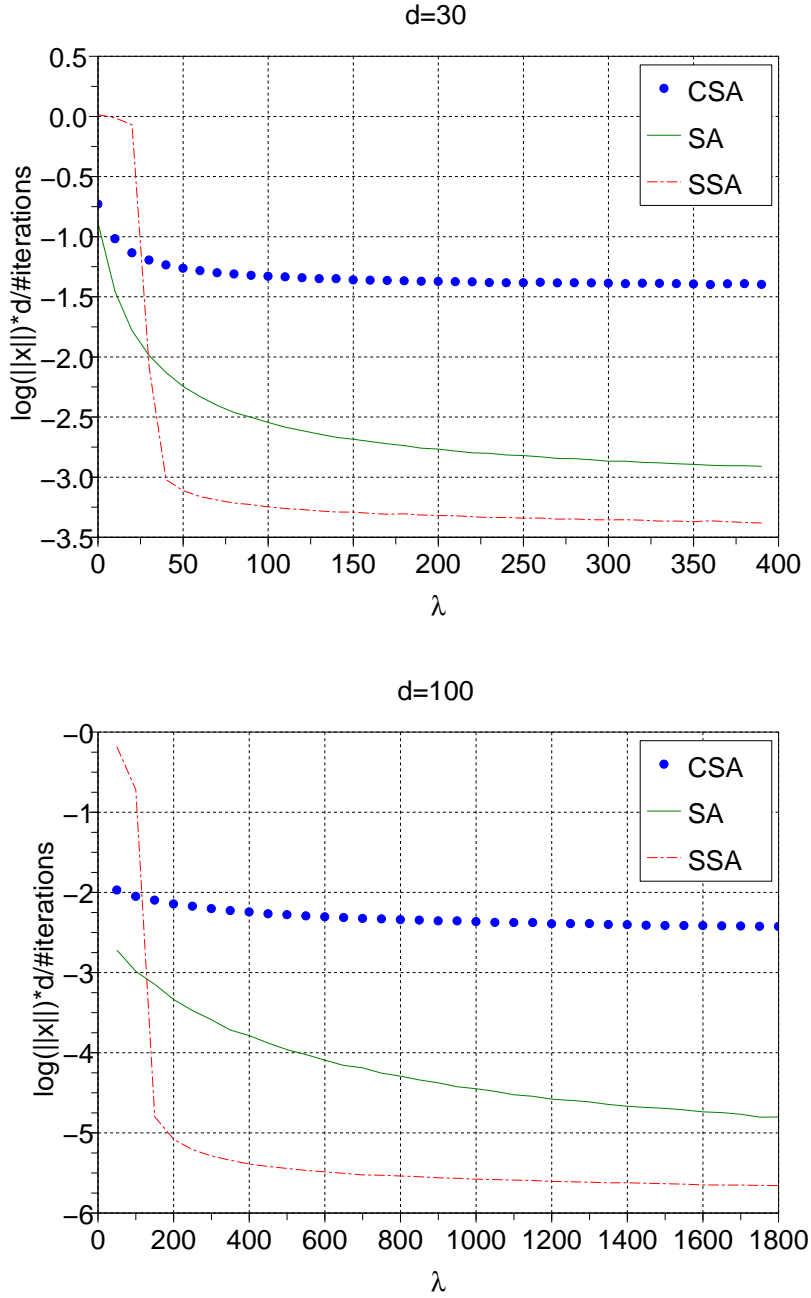
Figure 2.6: Log of distance to the optimum when the halting criterion ( f(x) < 10e^{-50} ) is met, normalized by the dimension and the number of iterations. Results for \mu = \lambda/2 , on the Sphere function in dimension 30 (Top) and dimension 100 (Bottom). In all cases, SSA is the best rule for \lambda large.
