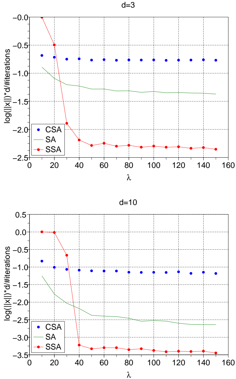
Figure 2.7: Results for \mu = \lambda/4 on the Sphere function in dimensions 3 (Top) and 10 (Bottom). All methods are better than for \mu = \lambda/2 . In all cases, SSA is the best rule for \lambda large.
