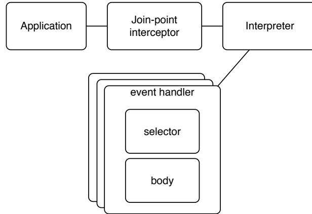
Figure 10.1 – Architecture of the EJAVA interpreter.
