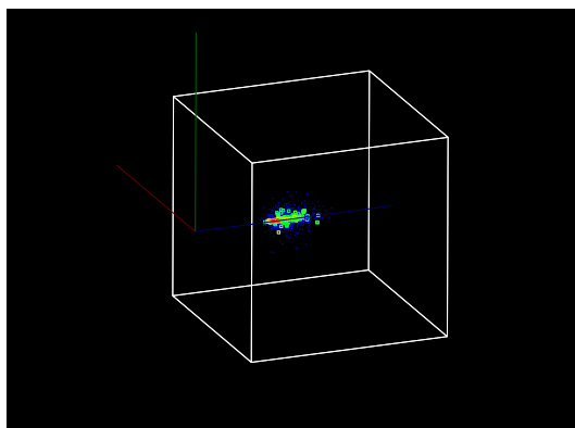
(b) Shower of a 20 GeV photon
