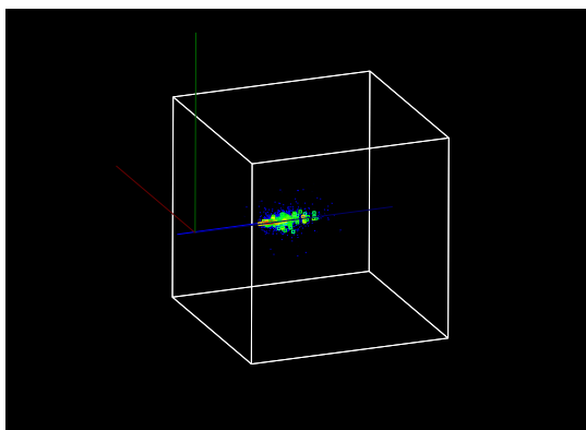
(a) Shower of a 20 GeV electron
