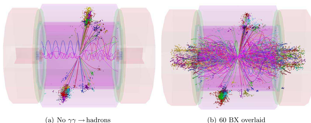
Figure 8.3: Illustration of the effect of \gamma\gamma \rightarrow hadrons event overlay on a 1 TeV Z^0 event over 60 BX in the CLIC ILD detector (taken from [87])
