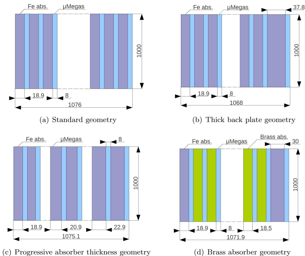
Figure 6.11: Scheme and summary of the considered alternative geometries.
