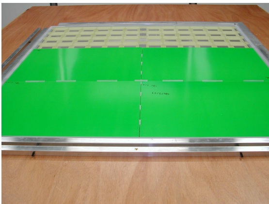
Figure 6.5: Photograph of the mechanical square meter prototype under assembly.
