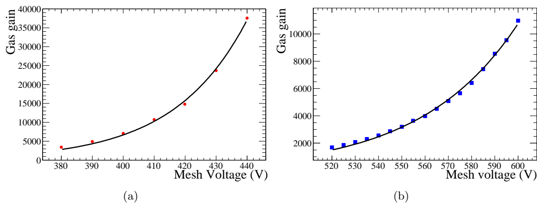
Figure 4.3: Gas gain versus mesh voltage fitted with the gas gain formula in Ar/ i\text{C}_4\text{H}_{10} (95/5) [4.3(a)] and in Ar/ \text{CO}_2 (80/20) [4.3(b)].
