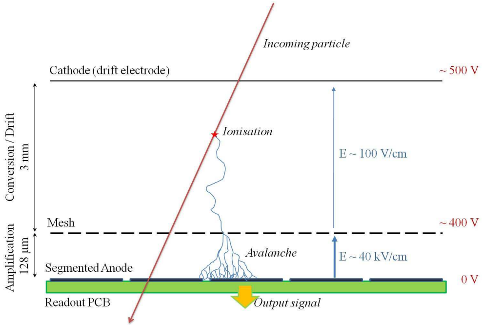
Figure 3.4: Scheme of MICROMEAS principle.
