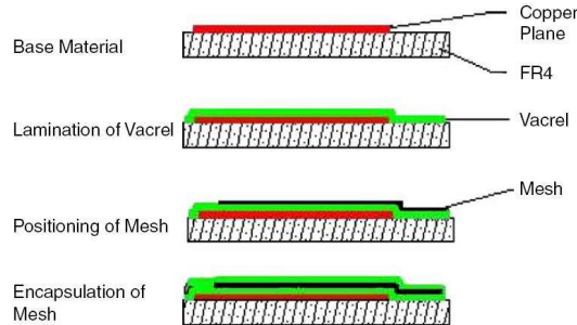
Figure 3.6: The MICROMEAS bulk fabrication process [51].
