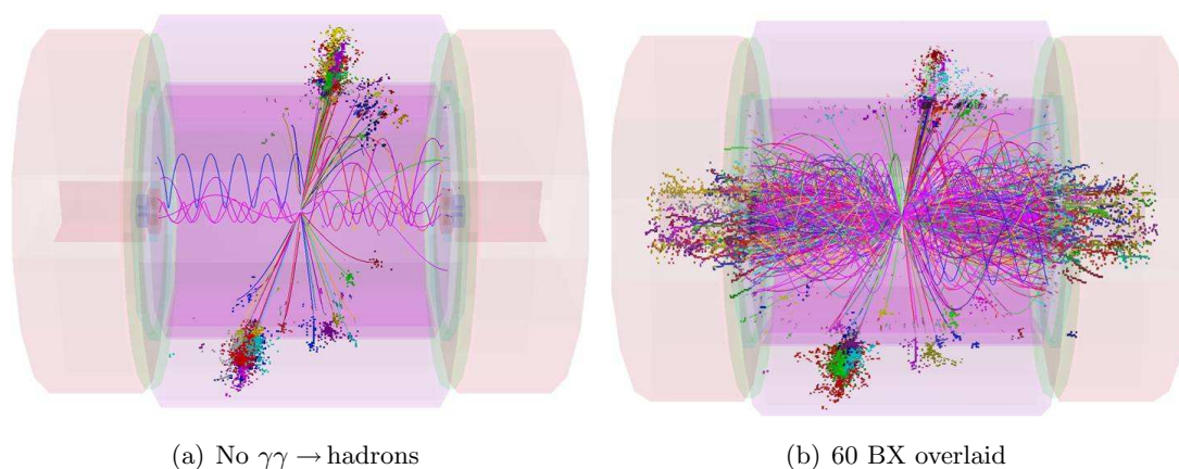
Figure 8.3: Illustration of the effect of \gamma\gamma \rightarrow \text{hadrons} event overlay on a 1 TeV Z^0 event over 60 BX in the CLIC ILD detector (taken from [87])
