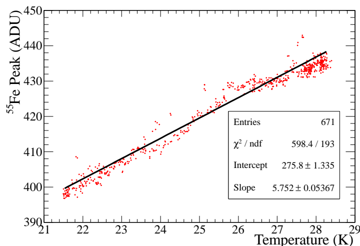
Figure 4.5: Pressure corrected ^{55}\text{Fe} peak value versus temperature.
