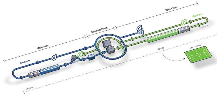
Figure 2.2: layout of the ILC machine.
