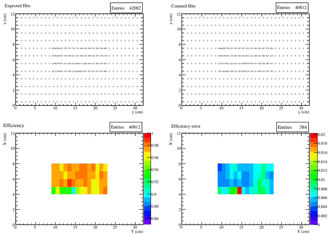
Figure 5.11: Efficiency map, principle of calculation.
