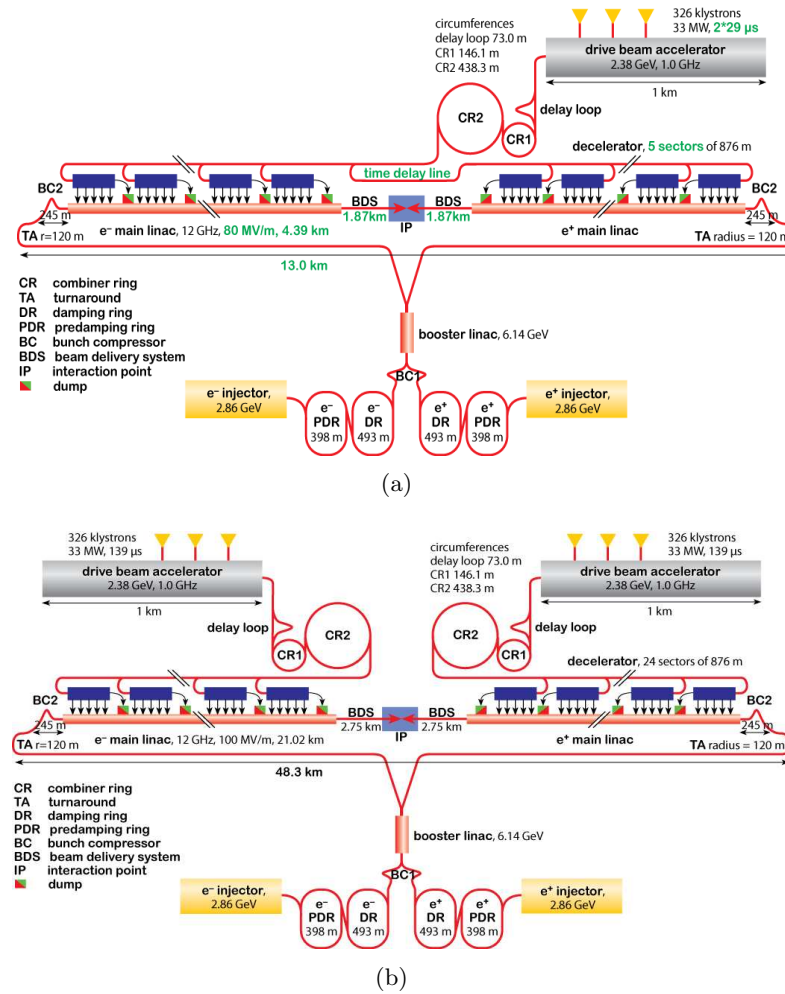
Figure 2.3: Layout of the low energy (a) and the nominal (b) version of the CLIC machine.
