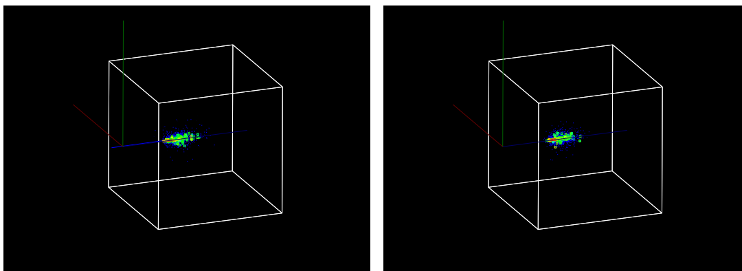
(a) Shower of a 20 GeV electron
