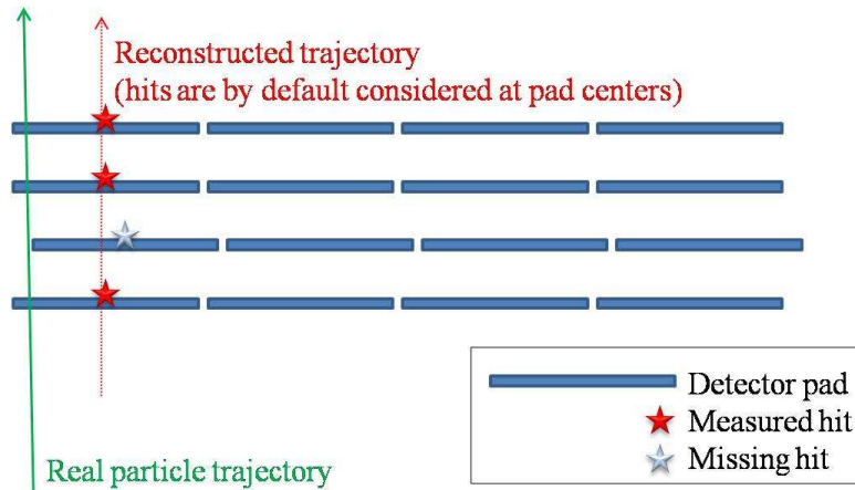
Figure 5.8: Geometrical inefficiency
