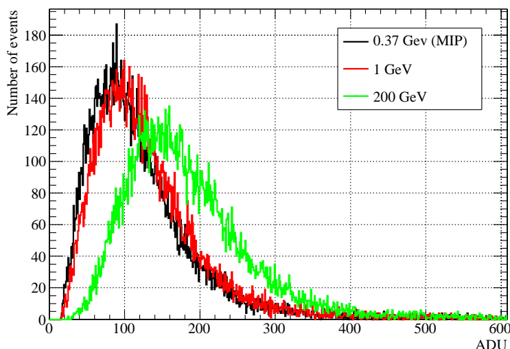
Figure 5.17: GEANT4 simulation of distribution of energy loss for muons crossing 3 mm of Ar/ i C 4 H 10 (95/5)
