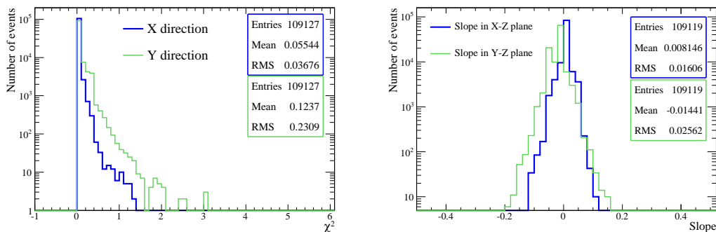
Figure 5.20: Straight line fit \chi^2 before applying cuts and slopes after the \chi^2 cut for all preselected events in the three small chambers (electron sample).
