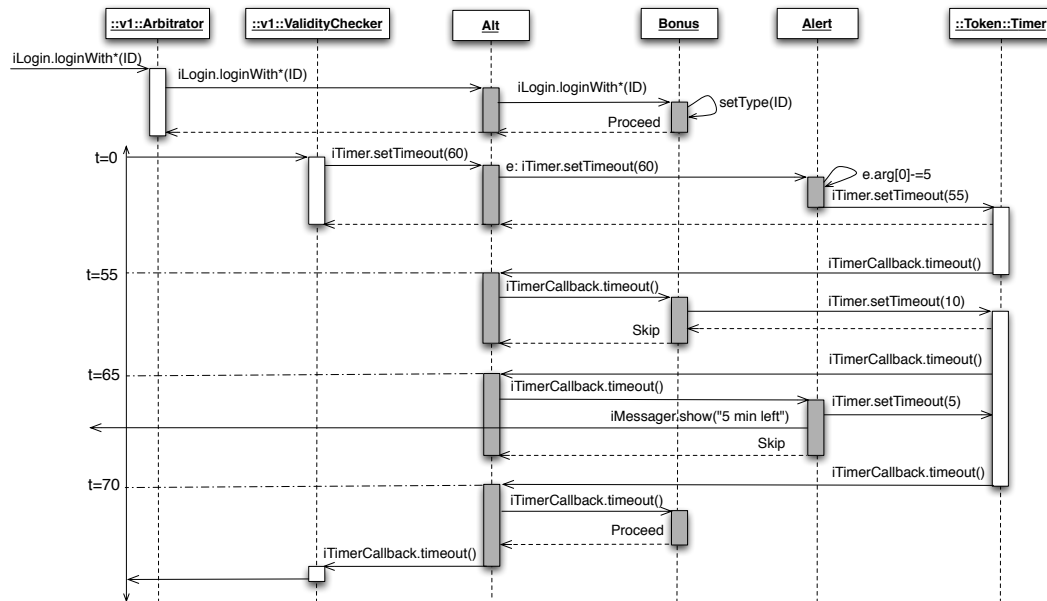
Figure 7.17: Alt(Bonus,Alert) scenario
