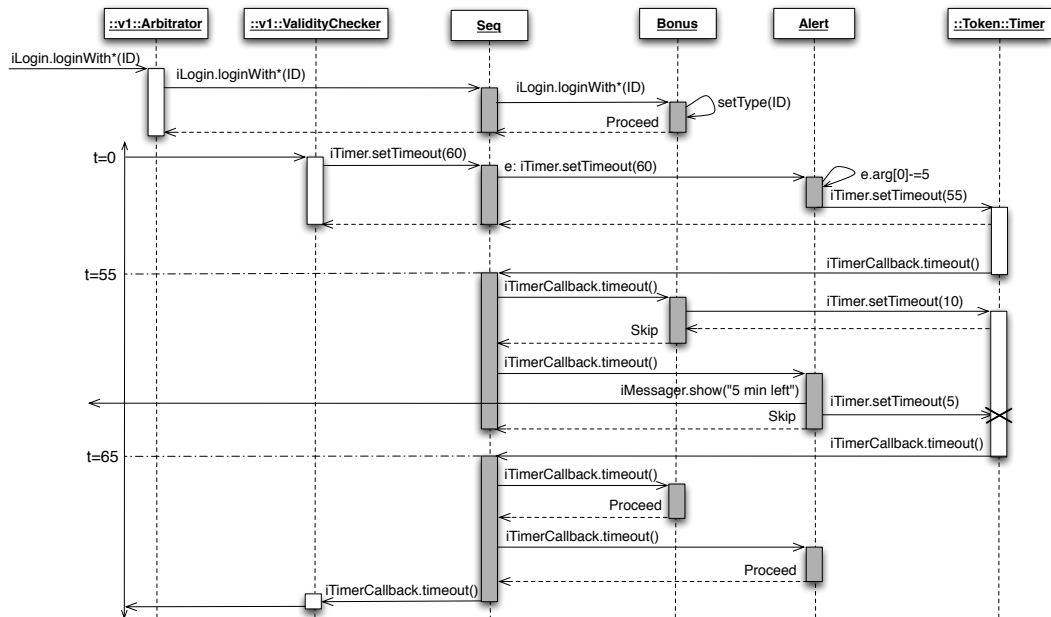
Figure 7.16: Seq(Bonus,Alert) scenario
