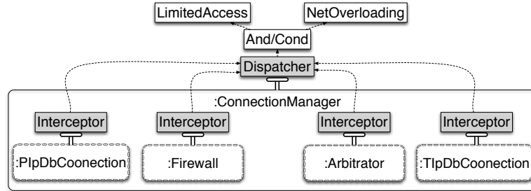
Figure 7.22: The view for LimitedAccess and NetOverloading aspects
