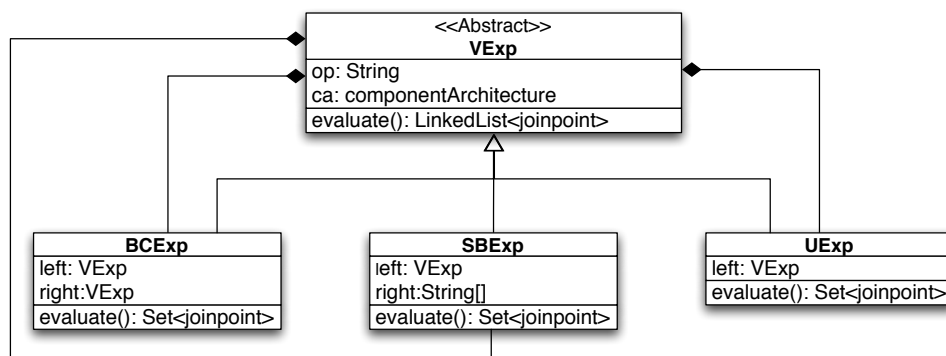
Figure 4.10: VIL Expressions structure
